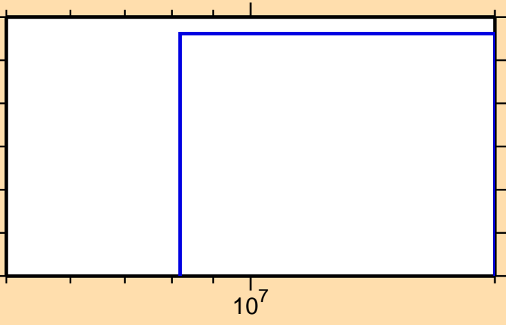
\sigma vs. E for ^{159}\text{Tm}(n,nt)
