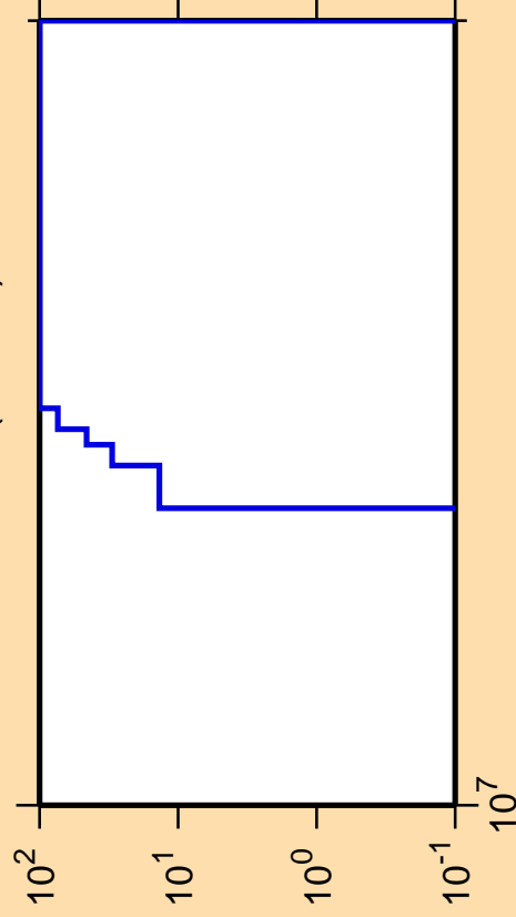
\Delta\sigma/\sigma vs. E for ^{160}\text{Tm} (mt117)
