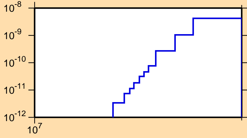
\sigma vs. E for ^{160}\text{Tm} (mt117)
