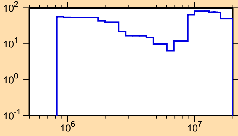
\Delta\sigma/\sigma vs. E for ^{160}\text{Tm}(n,n\text{cont.})
