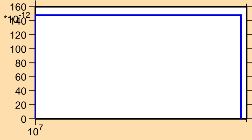
\sigma vs. E for ^{160}\text{Tm} (mt117)
