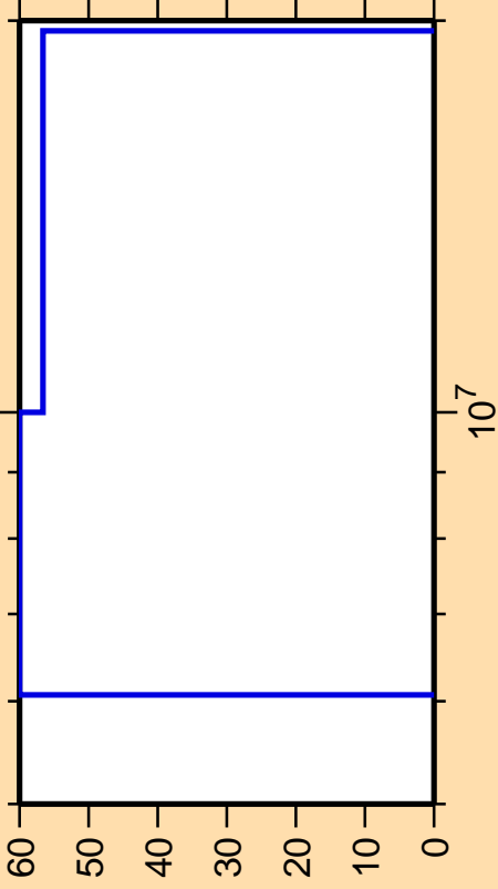
\Delta\sigma/\sigma vs. E for ^{160}\text{Tm}(n,p)
