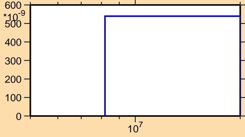
\sigma vs. E for ^{160}\text{Tm}(n,\text{He}3)
