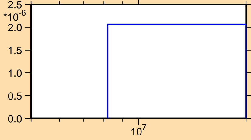
\sigma vs. E for ^{160}\text{Tm}(n,\text{nd})
