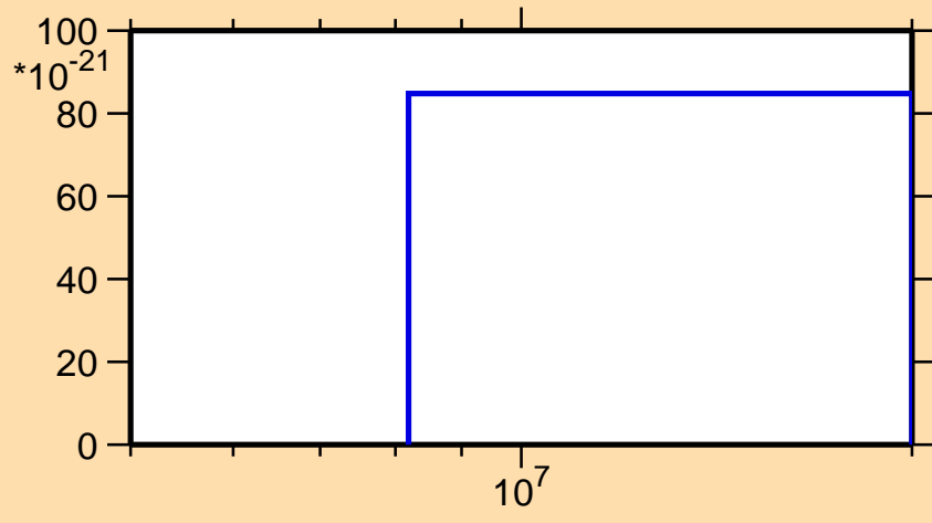
\sigma vs. E for ^{160}\text{Tm} (mt 11)
