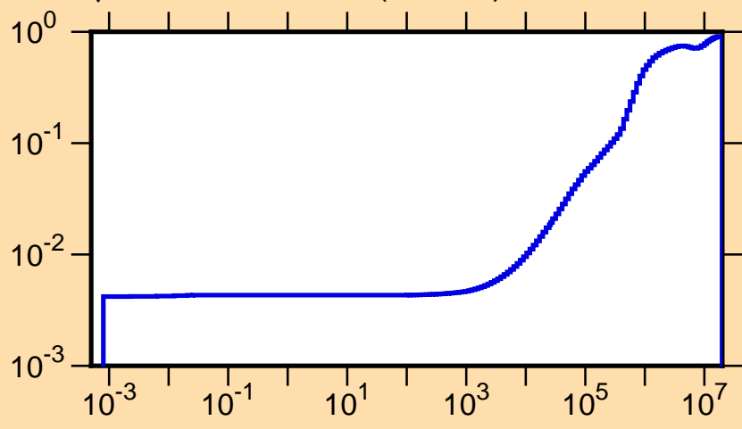
\mu vs. E for ^{161}\text{Tm}(\text{mt251})
