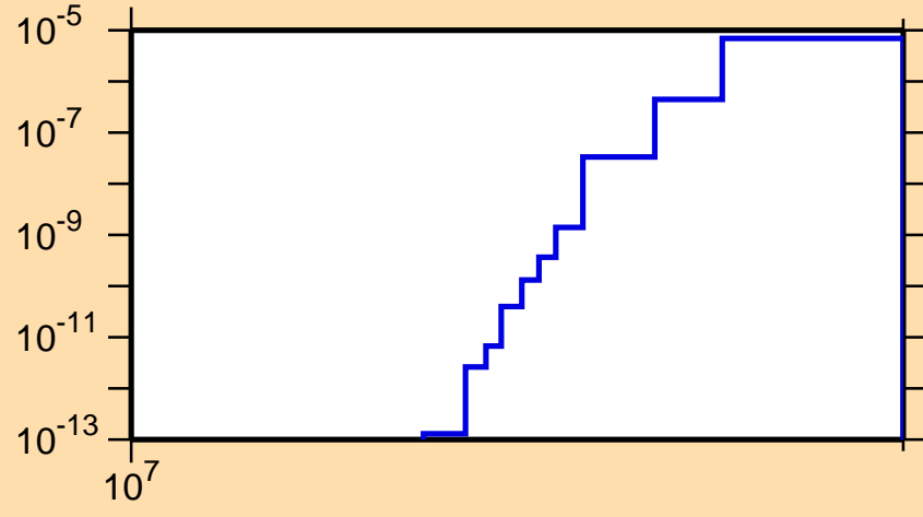
\sigma vs. E for ^{161}\text{Tm}(n,\text{nd})
