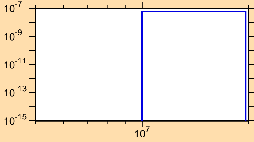
\sigma vs. E for ^{161}\text{Tm}(n,\text{He3})
