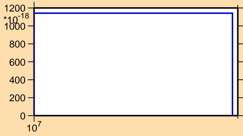
\sigma vs. E for ^{161}\text{Tm}(n,\text{pt})
