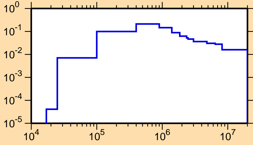
\sigma vs. E for ^{161}\text{Tm}(n,n_3)
