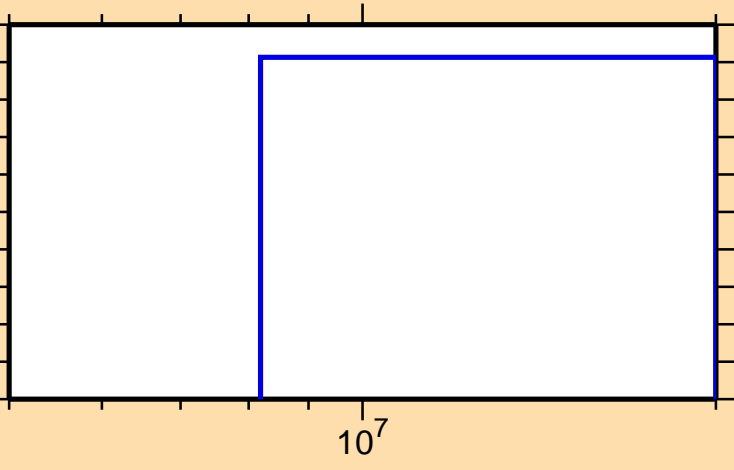
\sigma vs. E for ^{161}\text{Tm}(n,nt)
