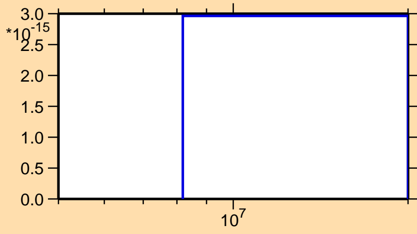
\sigma vs. E for ^{161}\text{Tm} (mt 34)
