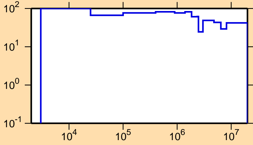
\Delta\sigma/\sigma vs. E for ^{161}\text{Tm}(n,n_1)
