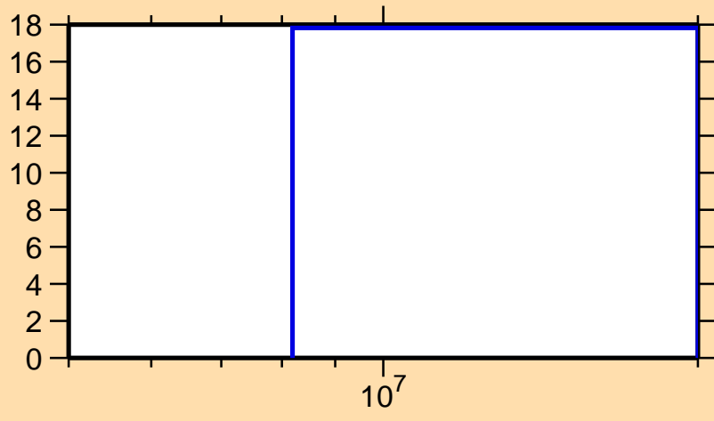
\Delta\sigma/\sigma vs. E for ^{161}\text{Tm}(n,\text{tot.})
