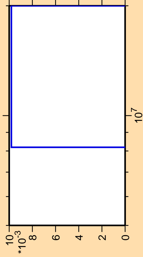
\Delta\sigma/\sigma vs. E for ^{161}\text{Tm}(n,\text{pt})
