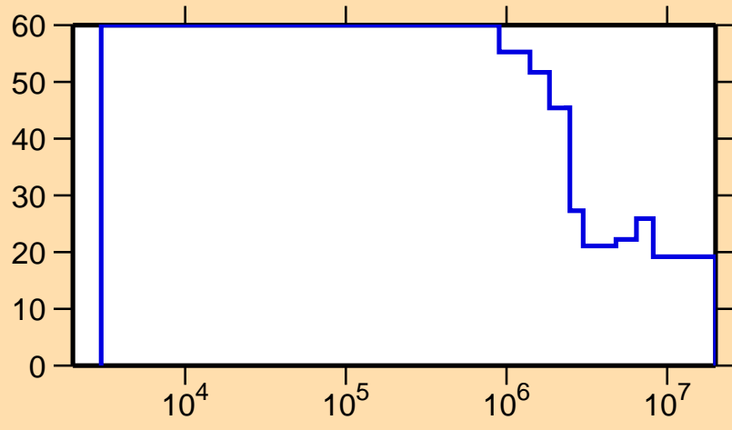
\Delta\sigma/\sigma vs. E for ^{161}\text{Tm}(n,\text{nonel.})
