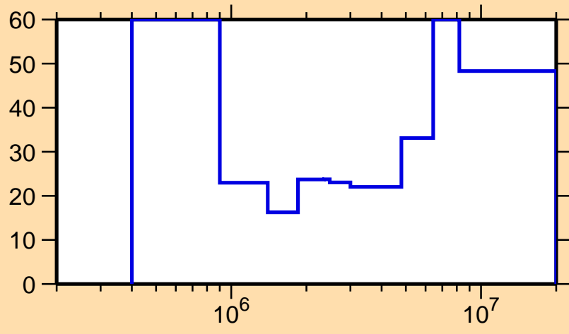
\Delta\sigma/\sigma vs. E for ^{161}\text{Tm}(n, el.)
