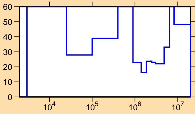
\Delta\sigma/\sigma vs. E for ^{161}\text{Tm}(n,\text{el.})
