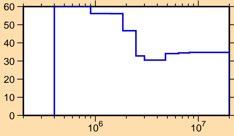
\Delta\sigma/\sigma vs. E for ^{161}\text{Tm}(n,n\text{cont.})
