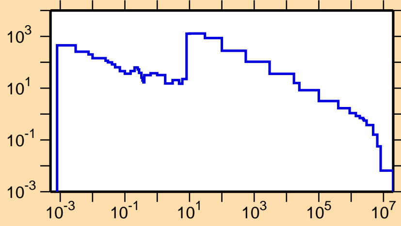
\sigma vs. E for ^{161}\text{Tm}(n,\gamma)
