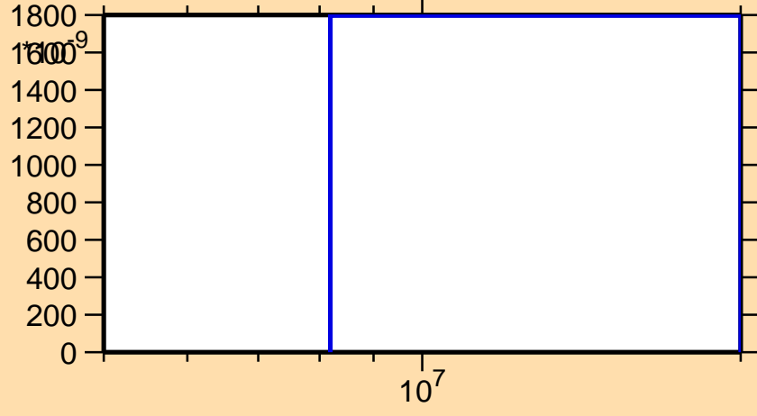
\sigma vs. E for ^{161}\text{Tm}(n,2np)
