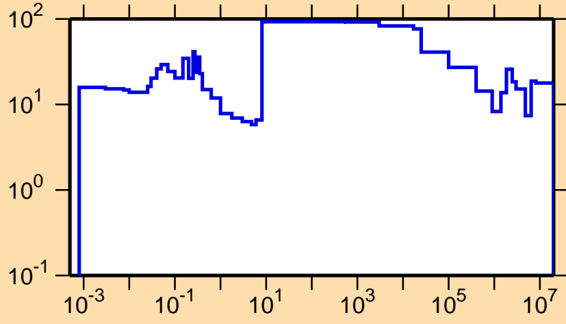
\Delta\sigma/\sigma vs. E for ^{161}\text{Tm}(n,\text{tot.})
