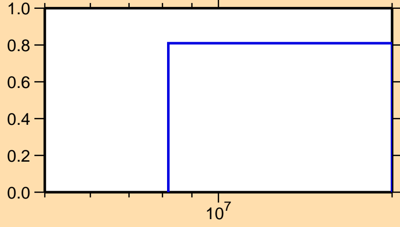
\sigma vs. E for ^{161}\text{Tm}(n,2n)
