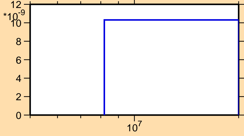
\sigma vs. E for ^{161}\text{Tm}(n,2n\alpha)
