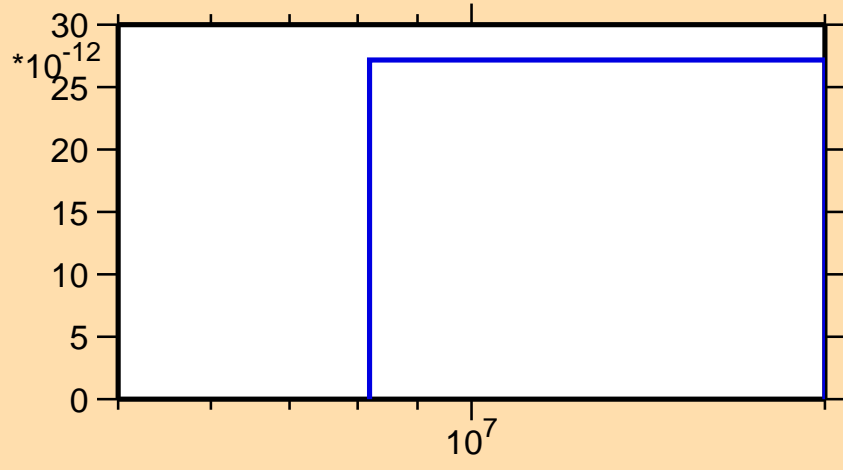
\sigma vs. E for ^{161}\text{Tm}(\text{mt117})
