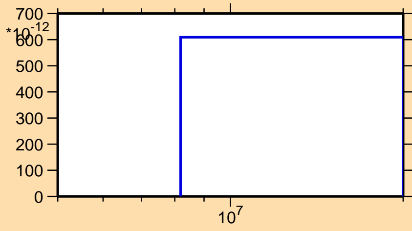
\sigma vs. E for ^{161}\text{Tm} (mt 45)
