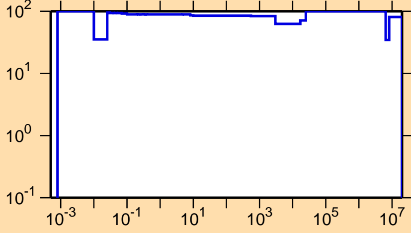
\Delta\sigma/\sigma vs. E for ^{161}\text{Tm}(n,p)
