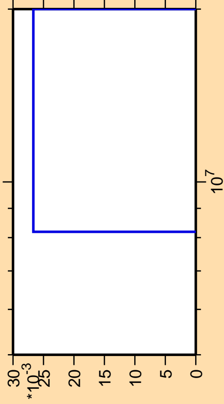
\Delta\sigma/\sigma vs. E for ^{161}\text{Tm} (mt 34)
