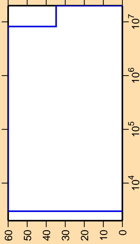
\Delta\sigma/\sigma vs. E for ^{161}\text{Tm}(n,\gamma)
