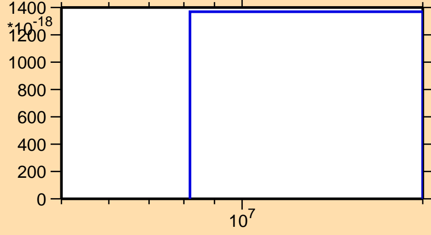
\sigma vs. E for ^{161}\text{Tm}(n,\text{pt})
