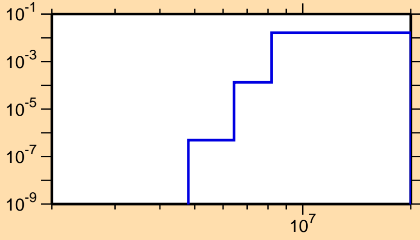
\sigma vs. E for ^{161}\text{Tm}(n,np)
