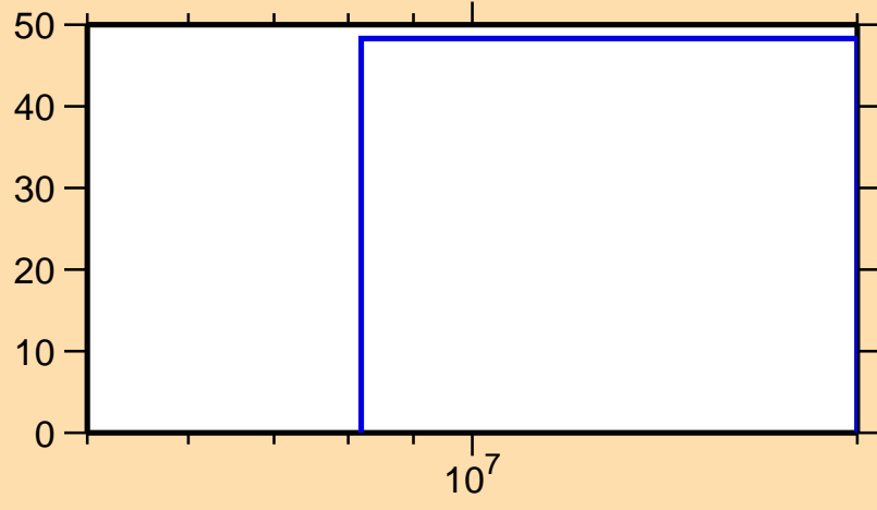
\Delta\sigma/\sigma vs. E for ^{161}\text{Tm}(n,\text{el.})
