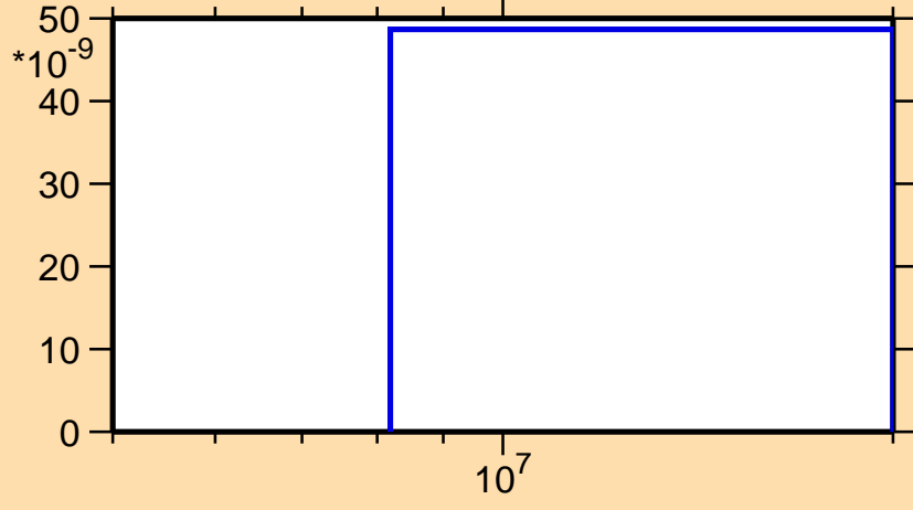
\sigma vs. E for ^{161}\text{Tm}(n,\text{He}3)
