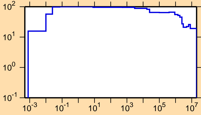
\Delta\sigma/\sigma vs. E for ^{161}\text{Tm}(n,\text{nonel.})
