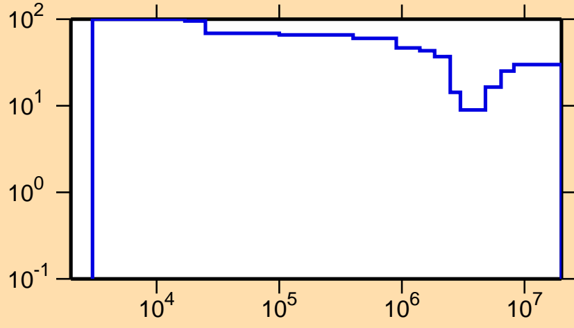
\Delta\sigma/\sigma vs. E for ^{161}\text{Tm}(n,\text{inel.})
