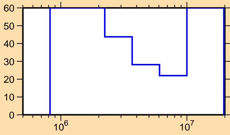
\Delta\sigma/\sigma vs. E for ^{162}\text{Tm}(n,n\text{cont.})
