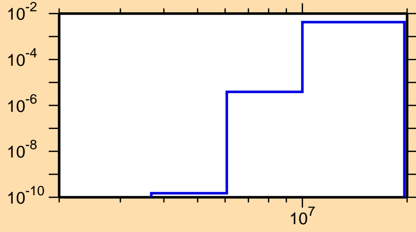
\sigma vs. E for ^{162}\text{Tm}(n,d)
