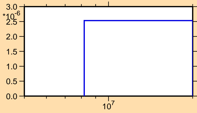
\sigma vs. E for ^{162}\text{Tm}(n,\text{nd})
