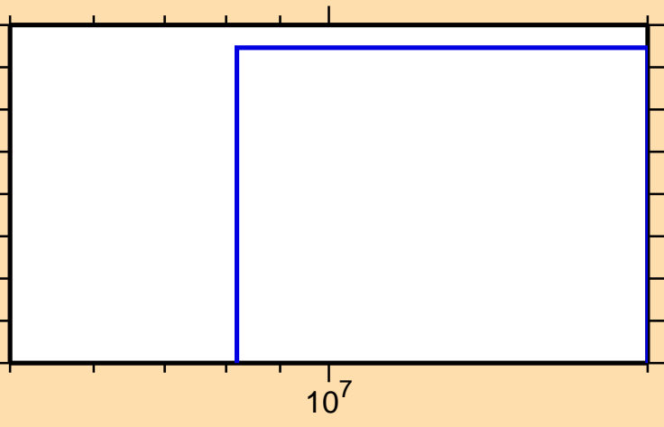
\sigma vs. E for ^{162}\text{Tm}(n,3n)
