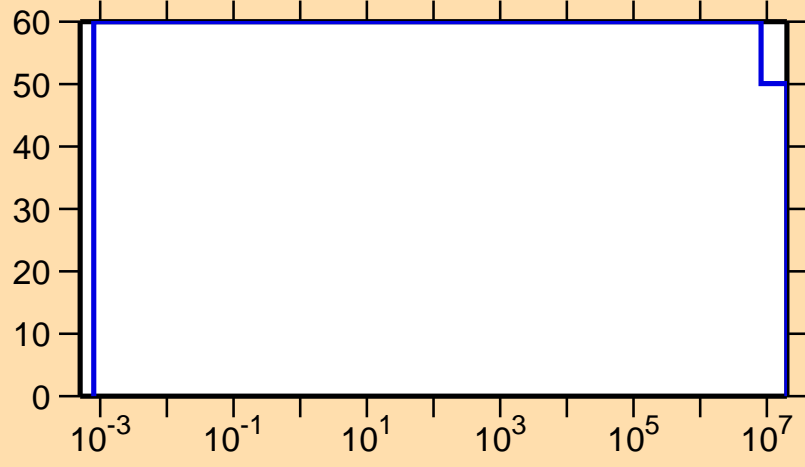
\Delta\sigma/\sigma vs. E for ^{162}\text{Tm}(n,p)
