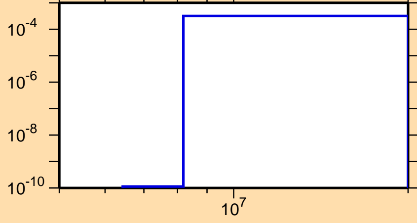
\sigma vs. E for ^{162}\text{Tm}(n,t)
