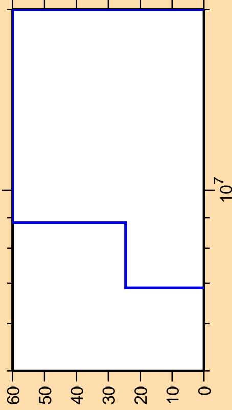
\Delta\sigma/\sigma vs. E for ^{162}\text{Tm}(n,n\text{cont.})
