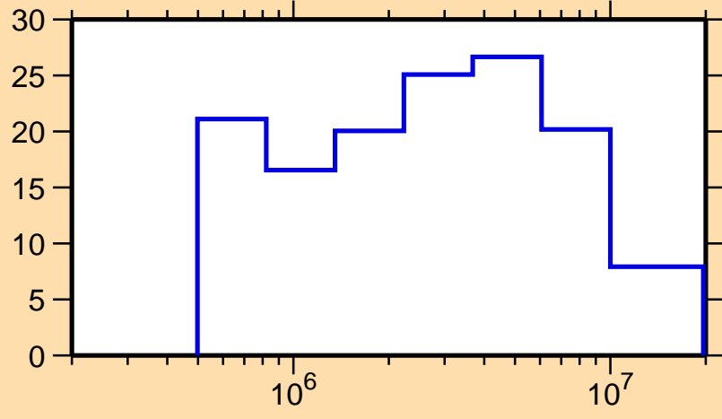
\Delta\sigma/\sigma vs. E for ^{162}\text{Tm}(n, el.)
