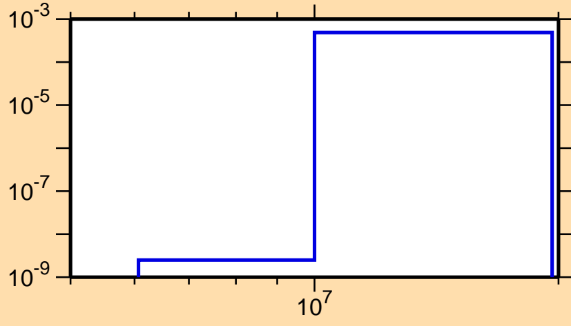
\sigma vs. E for ^{162}\text{Tm}(n,t)
