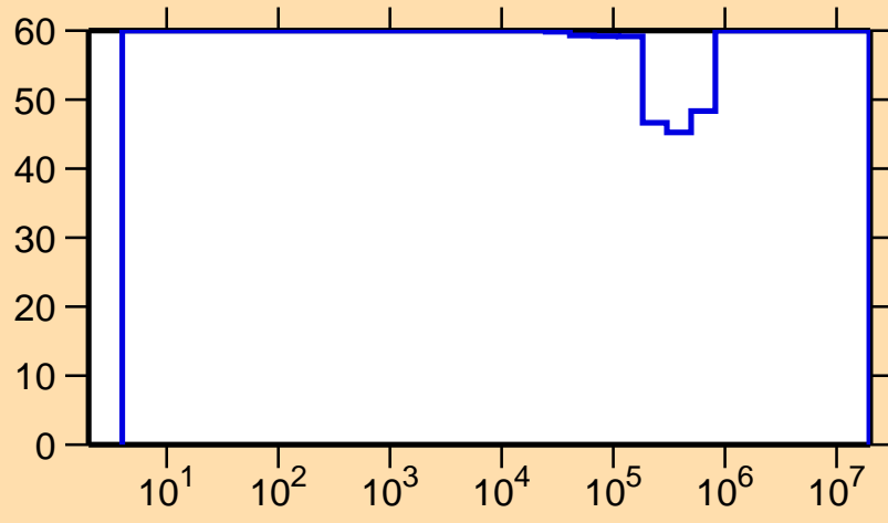
\Delta\sigma/\sigma vs. E for ^{162}\text{Tm}(n,n_1)
