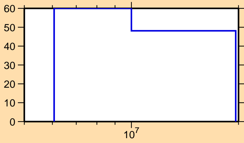
\Delta\sigma/\sigma vs. E for ^{162}\text{Tm}(n,2n)
