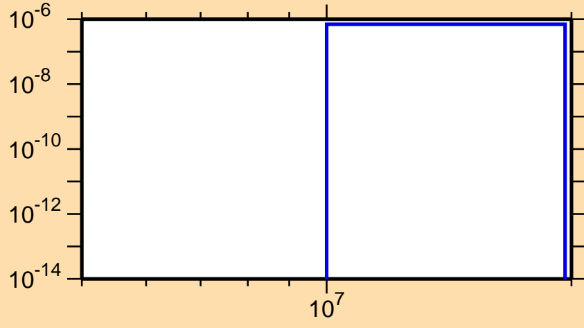
\sigma vs. E for ^{162}\text{Tm}(n,2n\alpha)
