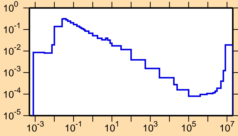
\sigma vs. E for ^{162}\text{Tm}(n,\alpha)
