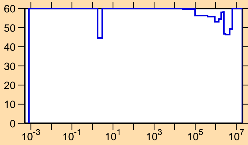
\Delta\sigma/\sigma vs. E for ^{162}\text{Tm}(n,\gamma)
