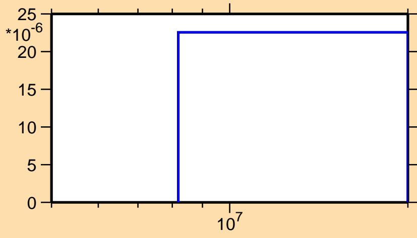
\sigma vs. E for ^{162}\text{Tm}(n,3n)
