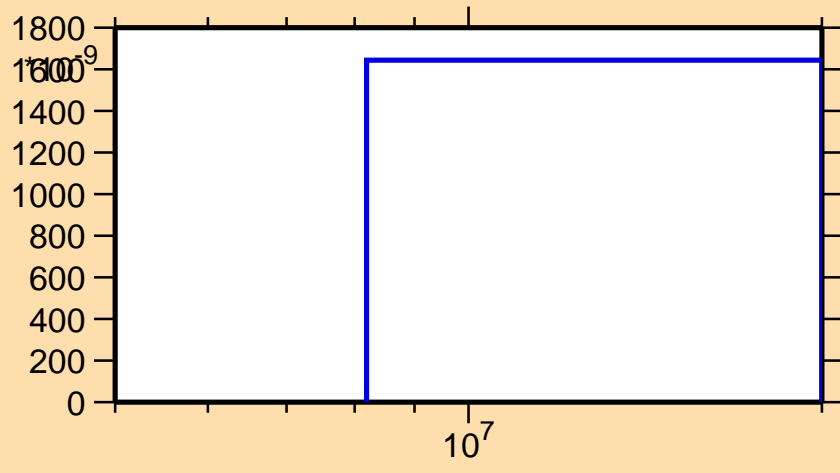
\sigma vs. E for ^{162}\text{Tm}(n,nd)
