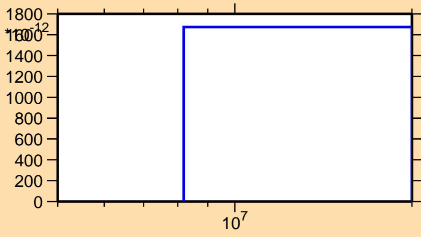
\sigma vs. E for ^{162}\text{Tm}(n,nt)
