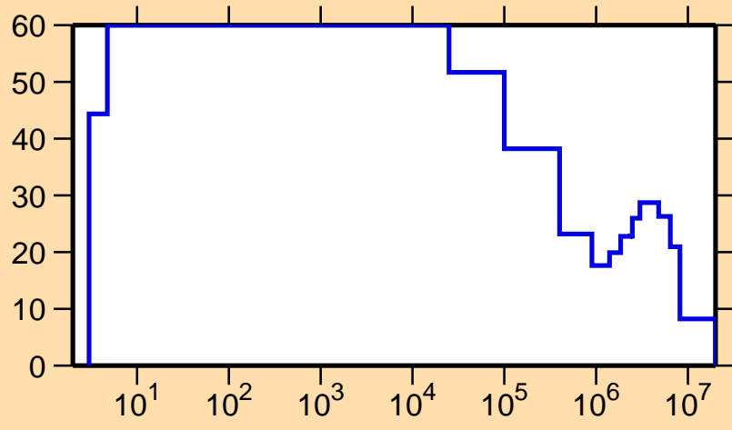
\Delta\sigma/\sigma vs. E for ^{162}\text{Tm}(n,\text{el.})
