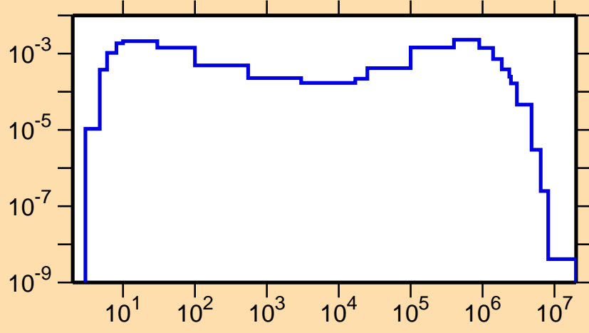
\sigma vs. E for ^{162}\text{Tm}(n,n_2)
