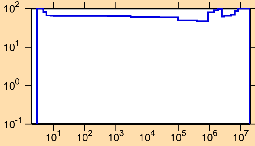
\Delta\sigma/\sigma vs. E for ^{162}\text{Tm}(n,n_1)
