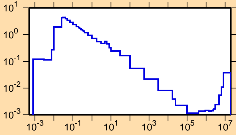
\sigma vs. E for ^{162}\text{Tm}(n,p)
