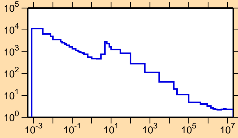
\sigma vs. E for ^{162}\text{Tm}(n,\text{nonel.})
