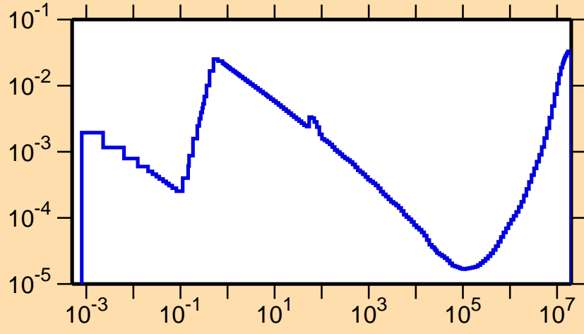
\sigma vs. E for ^{163}\text{Tm}(n,p)
