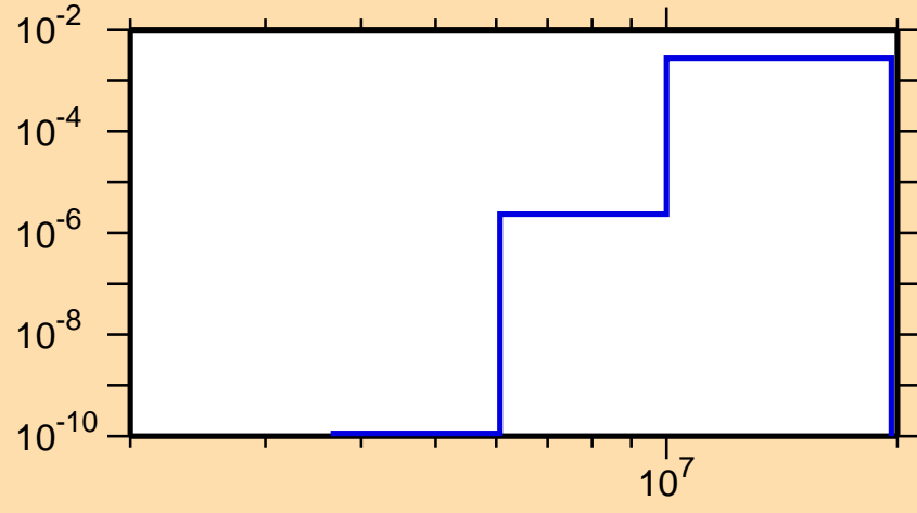
\sigma vs. E for ^{163}\text{Tm}(n,d)
