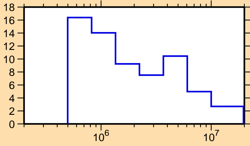
\Delta\sigma/\sigma vs. E for ^{163}\text{Tm}(n,\text{tot.})
