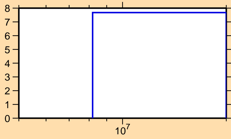
\Delta\sigma/\sigma vs. E for ^{163}\text{Tm}(n,\text{nonel.})
