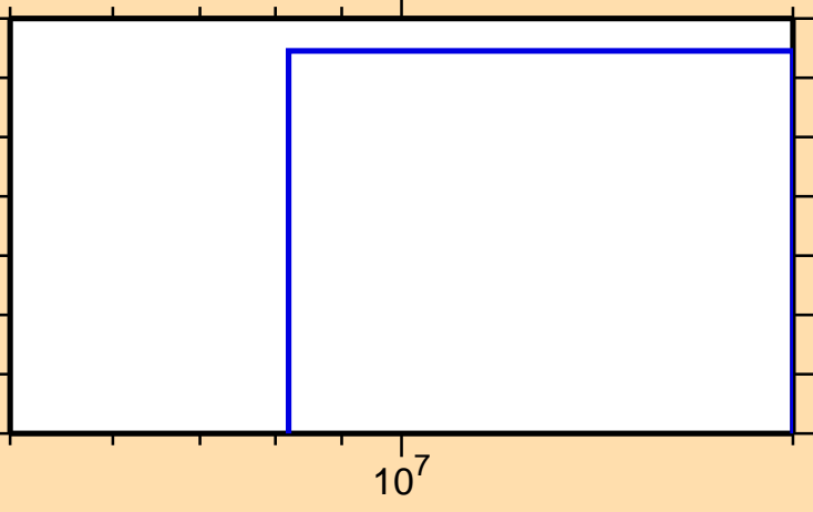
\sigma vs. E for ^{163}\text{Tm}(n,2n\alpha)
