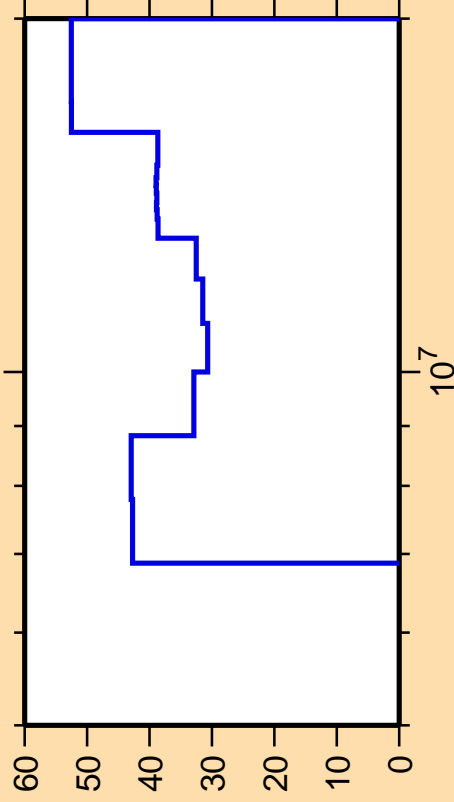
\Delta\sigma/\sigma vs. E for ^{164}\text{Tm}(n,\gamma)
