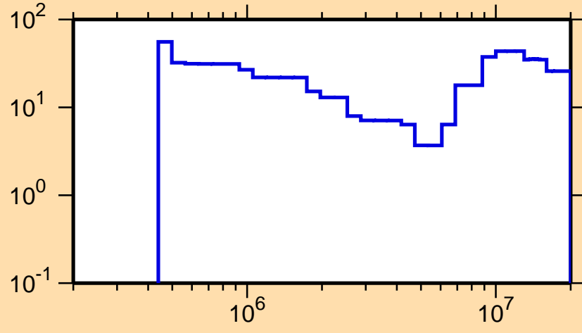
\Delta\sigma/\sigma vs. E for ^{164}\text{Tm}(n,n\text{cont.})
