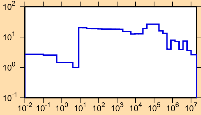
\Delta\sigma/\sigma vs. E for ^{164}\text{Tm}(n,el.)
