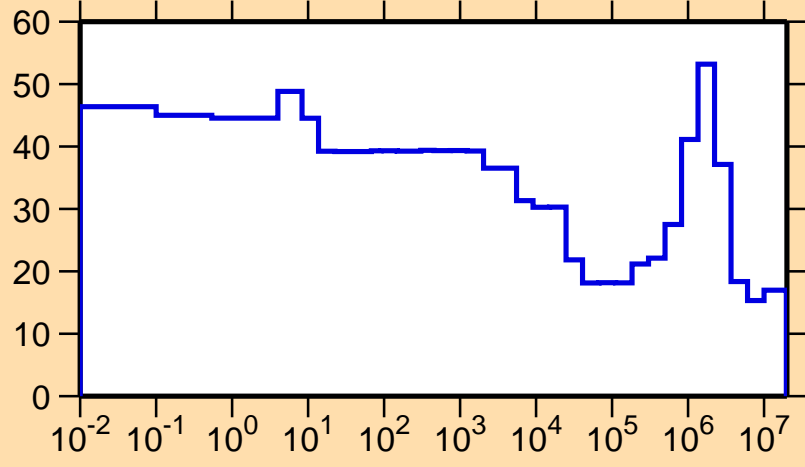
\Delta\sigma/\sigma vs. E for ^{164}\text{Tm}(n,p)
