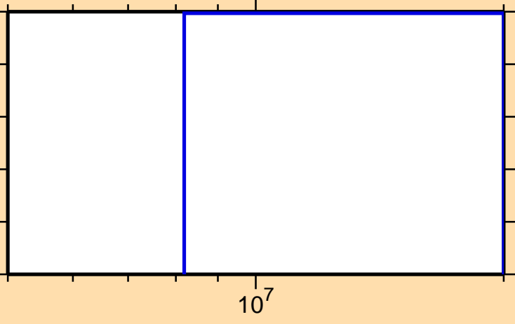
\sigma vs. E for ^{164}\text{Tm}(n,2np)
