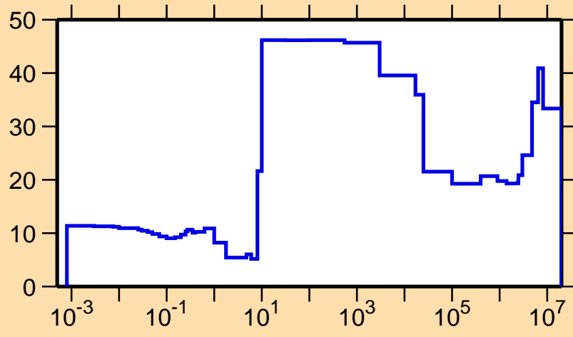
\Delta\sigma/\sigma vs. E for ^{164}\text{Tm}(n,\gamma)
