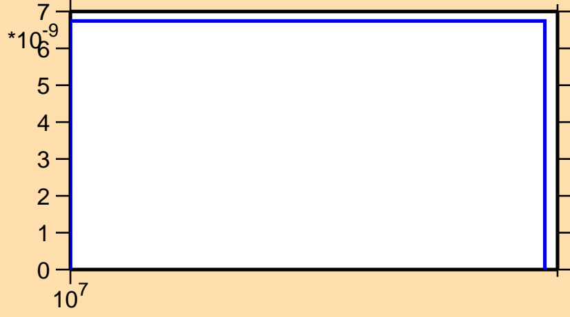
\sigma vs. E for ^{166}\text{Tm}(n,nt)
