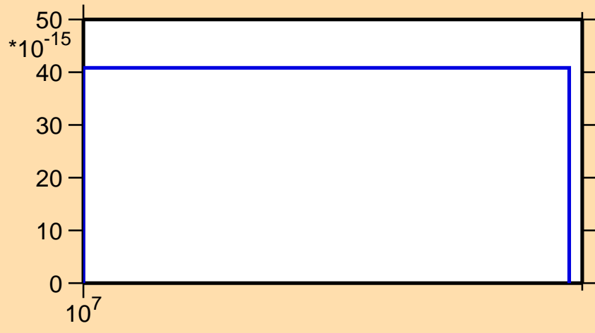
\sigma vs. E for ^{166}\text{Tm} (mt 45)
