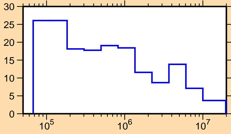
\Delta\sigma/\sigma vs. E for ^{166}\text{Tm}(n,\text{tot.})
