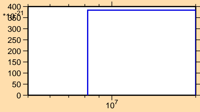
\sigma vs. E for ^{166}\text{Tm} (mt 11)
