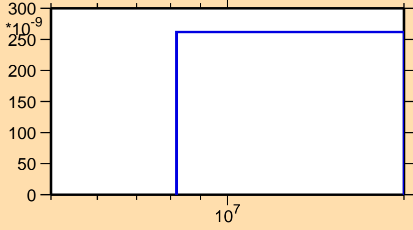
\sigma vs. E for ^{166}\text{Tm}(n,2n\alpha)
