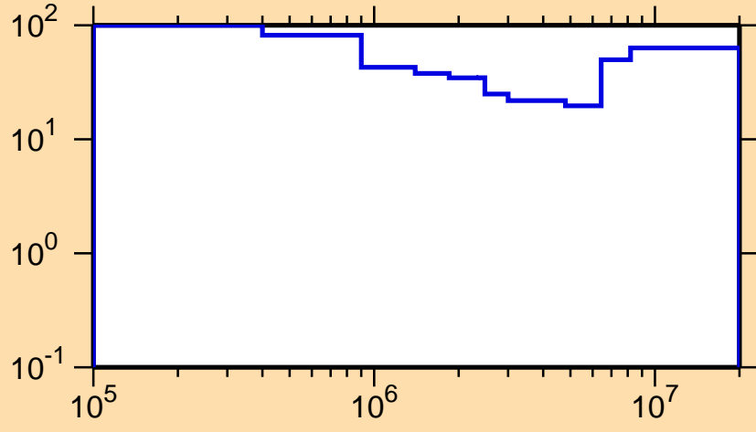
\Delta\sigma/\sigma vs. E for ^{166}\text{Tm}(n,ncont.)
