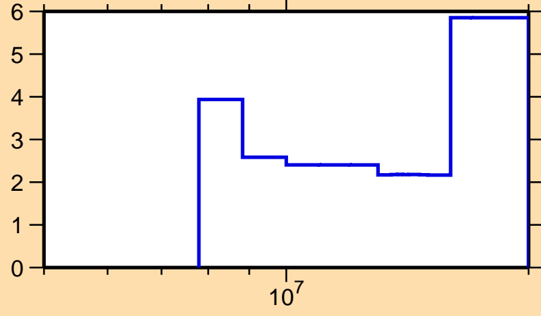
\Delta\sigma/\sigma vs. E for ^{167}\text{Tm}(n,\text{tot.})
