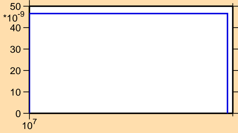
\sigma vs. E for ^{167}\text{Tm}(n,nd)
