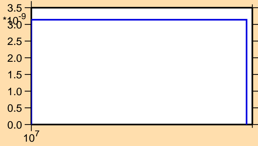
\sigma vs. E for ^{167}\text{Tm}(n,2n\alpha)
