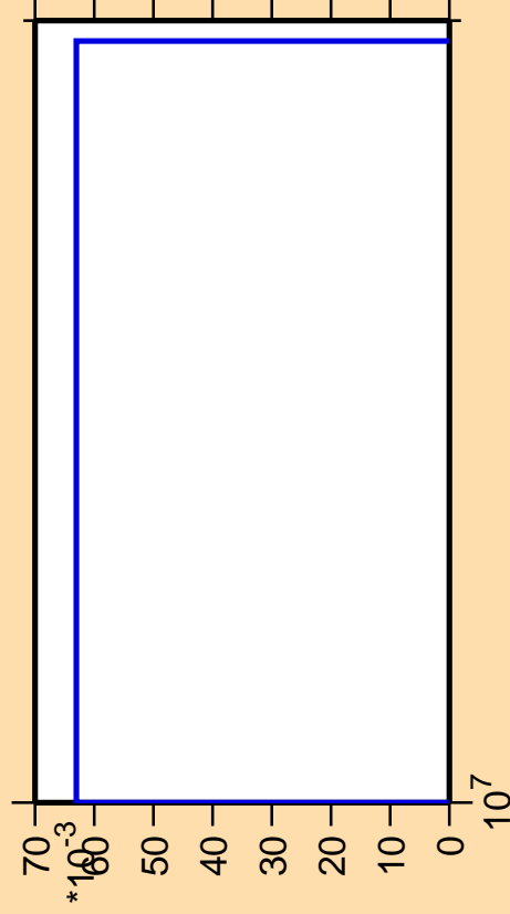
\Delta\sigma/\sigma vs. E for ^{167}\text{Tm} (mt 45)
