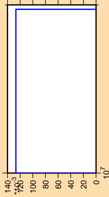
\Delta\sigma/\sigma vs. E for ^{167}\text{Tm}(\text{mt117})
