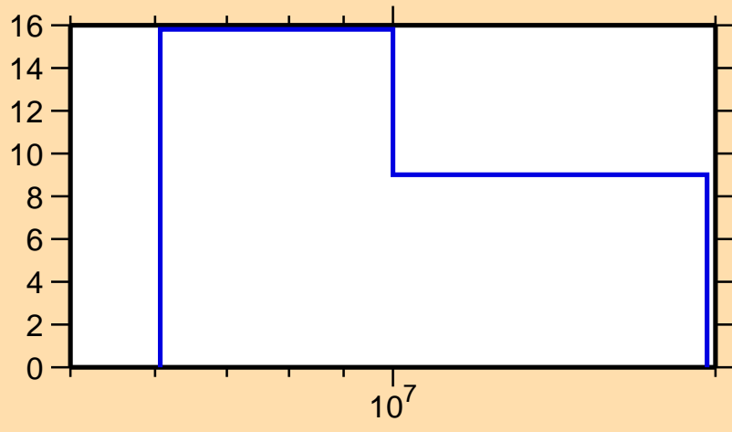
\Delta\sigma/\sigma vs. E for ^{167}\text{Tm}(n,2n)
