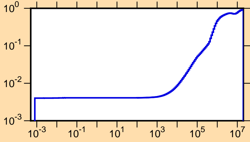
\mu vs. E for ^{168}\text{Tm}(\text{mt251})
