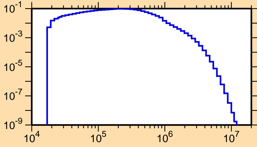
\sigma vs. E for ^{168}\text{Tm}(n,n_2)
