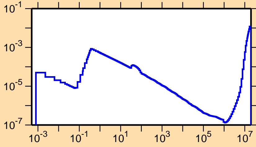
\sigma vs. E for ^{168}\text{Tm}(n,\alpha)
