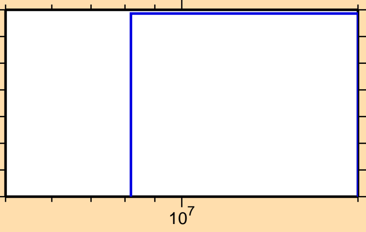
\sigma vs. E for ^{168}\text{Tm}(n,3n)
