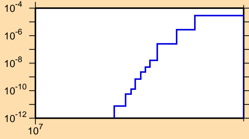
\sigma vs. E for ^{170}\text{Tm}(n,nd)
