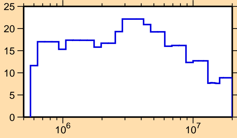
\Delta\sigma/\sigma vs. E for ^{170}\text{Tm}(n,el.)
