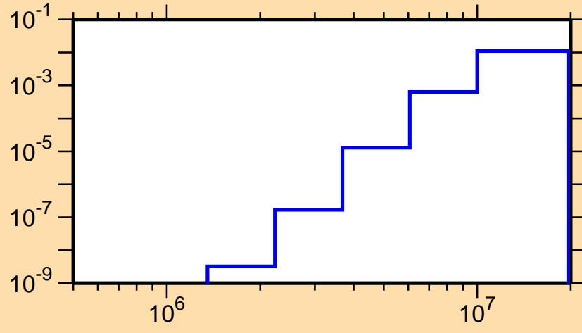
\sigma vs. E for ^{170}\text{Tm}(n,p)
