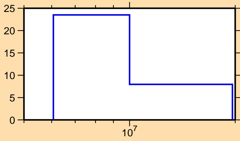
\Delta\sigma/\sigma vs. E for ^{170}\text{Tm}(n,2n)
