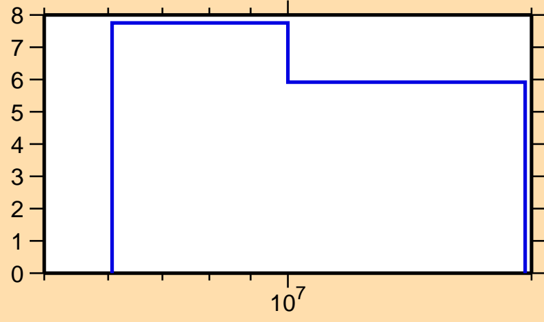
\Delta\sigma/\sigma vs. E for ^{170}\text{Tm}(n,\text{nonel.})
