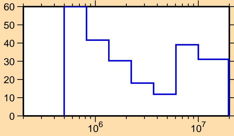
\Delta\sigma/\sigma vs. E for ^{170}\text{Tm}(n,n\text{cont.})
