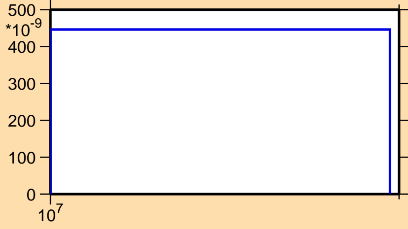
\sigma vs. E for ^{170}\text{Tm}(n,nd)
