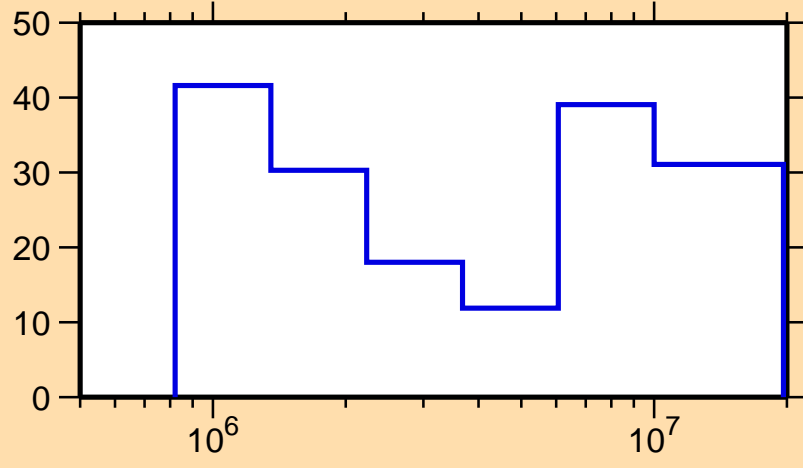
\Delta\sigma/\sigma vs. E for ^{170}\text{Tm}(n,ncont.)
