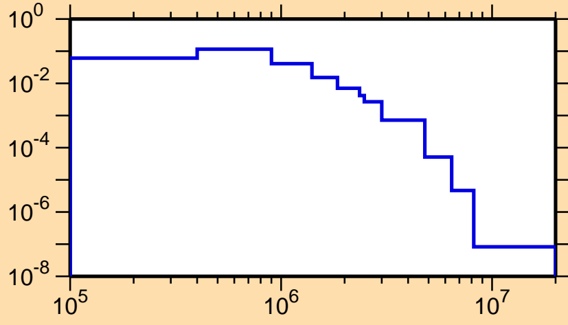
\sigma vs. E for ^{170}\text{Tm}(n,n_4)
