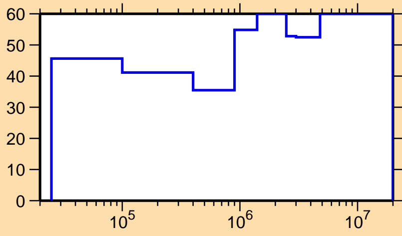
\Delta\sigma/\sigma vs. E for ^{170}\text{Tm}(n,n_1)
