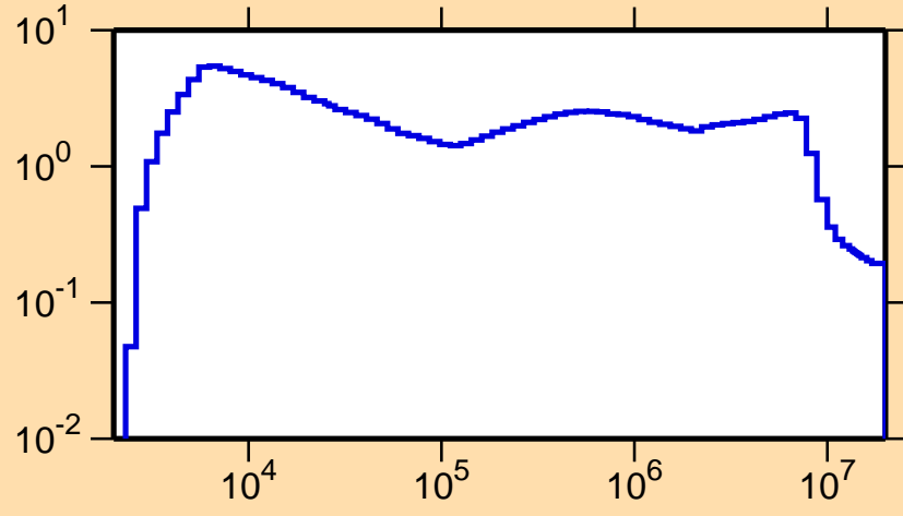
\sigma vs. E for ^{173}\text{Tm}(n,\text{inel.})
