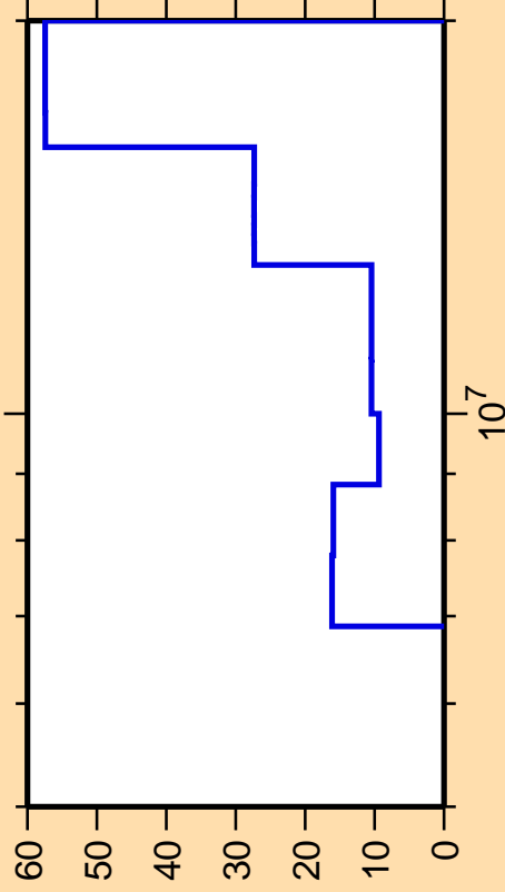
\Delta\sigma/\sigma vs. E for ^{173}\text{Tm}(n,2n)
