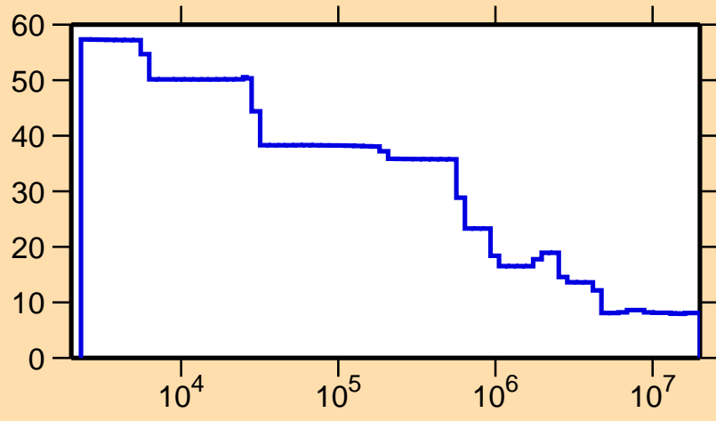
\Delta\sigma/\sigma vs. E for ^{173}\text{Tm}(n,\text{nonel.})
