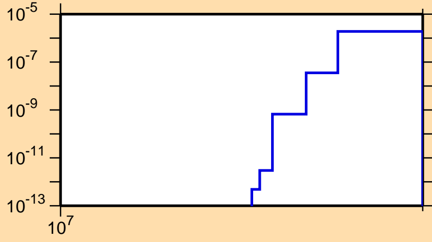
\sigma vs. E for ^{173}\text{Tm}(n,nt)
