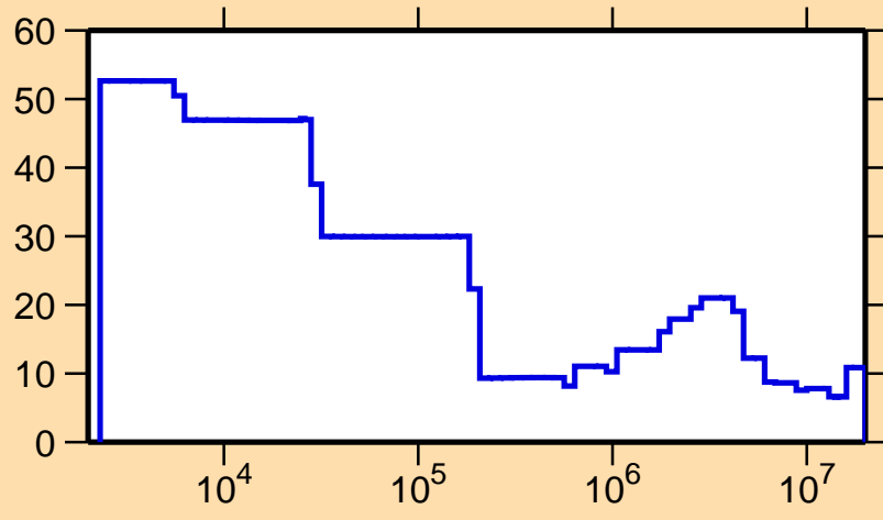
\Delta\sigma/\sigma vs. E for ^{173}\text{Tm}(n,\text{el.})
