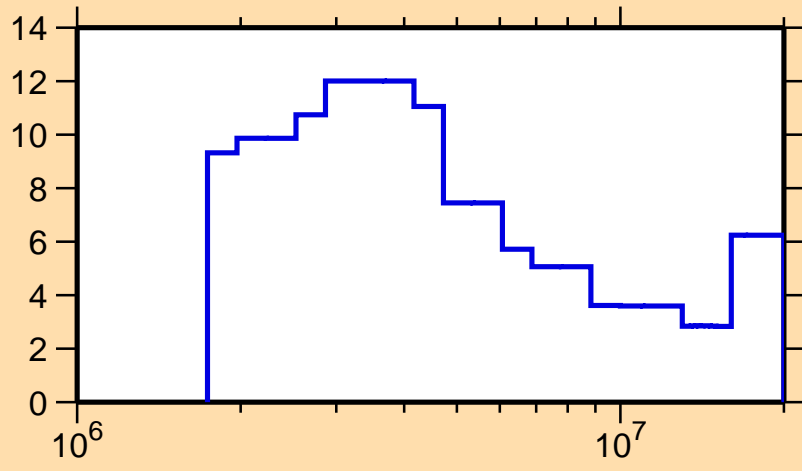
\Delta\sigma/\sigma vs. E for ^{173}\text{Tm}(n,\text{tot.})
