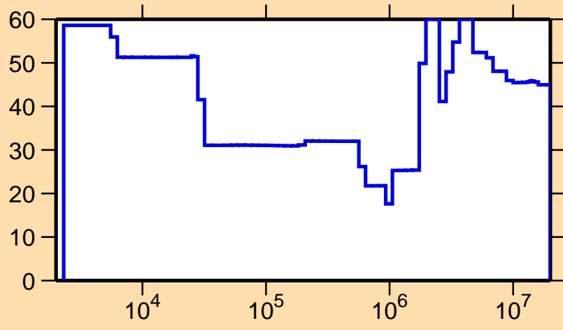
\Delta\sigma/\sigma vs. E for ^{173}\text{Tm}(n,n_1)
