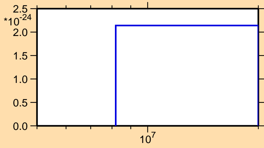
\sigma vs. E for ^{173}\text{Tm} (mt 42)
