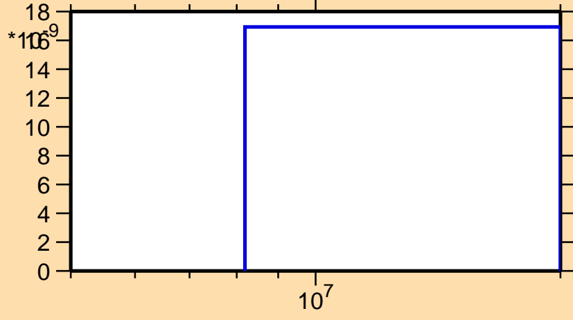
\sigma vs. E for ^{173}\text{Tm}(n,nt)
