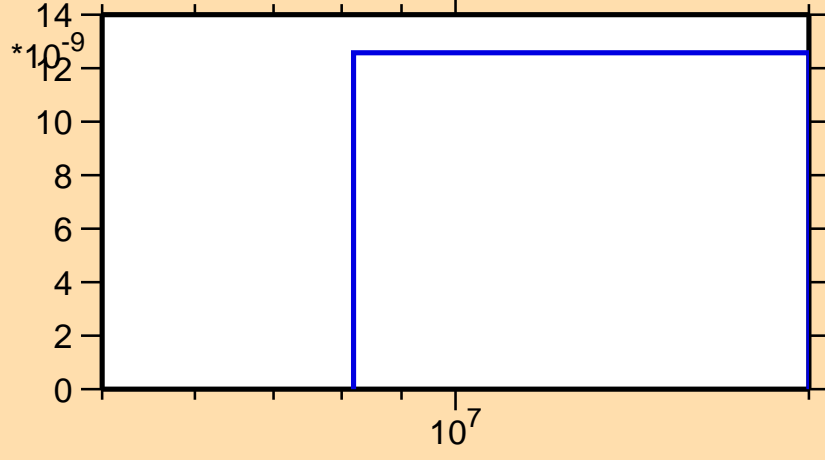
\sigma vs. E for ^{173}\text{Tm}(n,nd)
