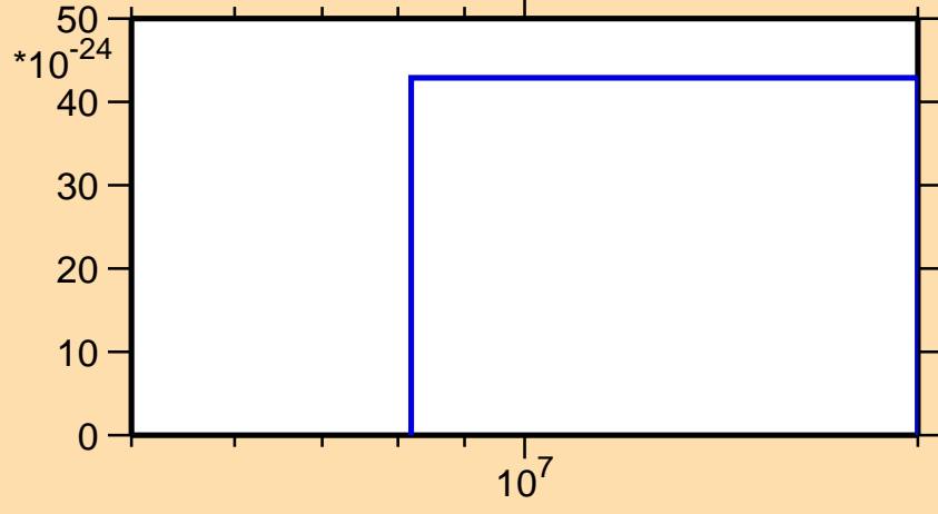
\sigma vs. E for ^{174}\text{Tm} (mt 42)
