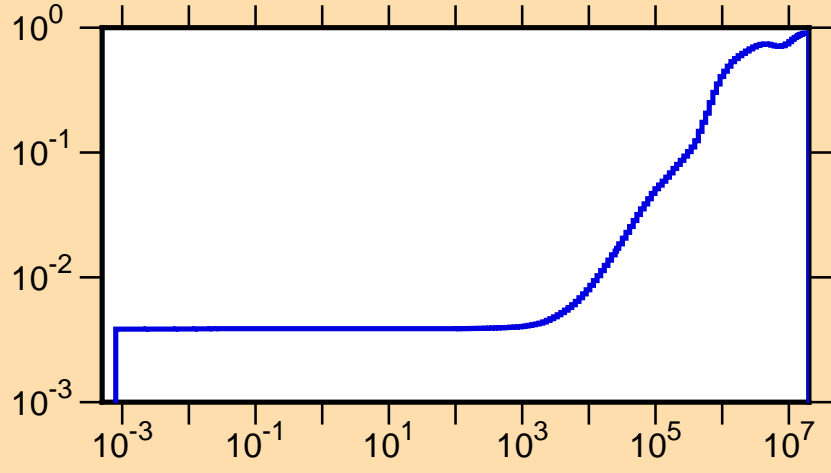
\mu vs. E for ^{175}\text{Tm}(\text{mt251})
