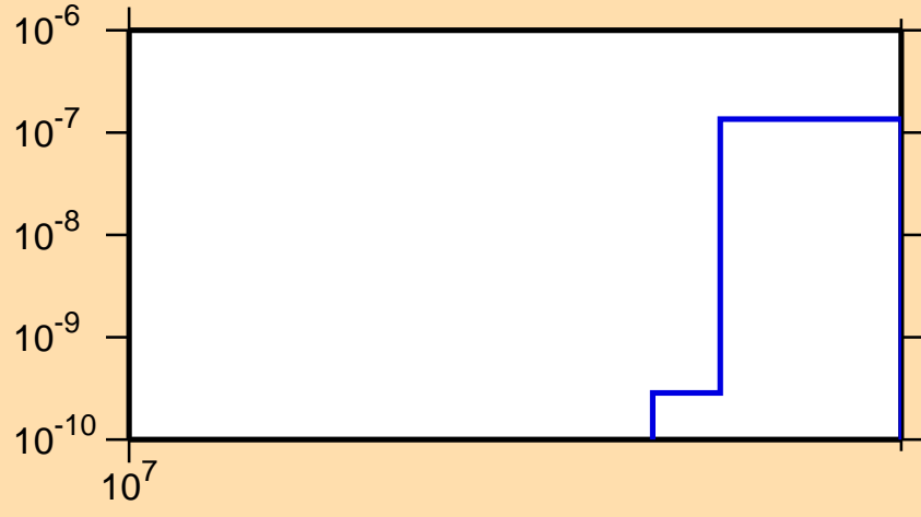
\sigma vs. E for ^{175}\text{Tm}(n,2np)
