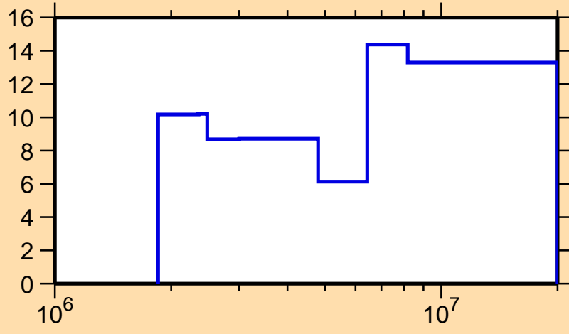
\Delta\sigma/\sigma vs. E for ^{175}\text{Tm}(n,inel.)
