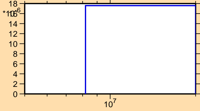
\sigma vs. E for ^{175}\text{Tm}(n,t)
