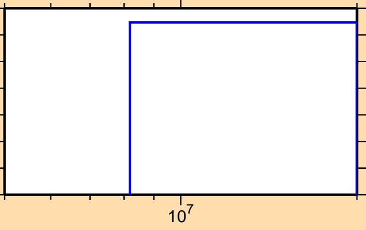
\sigma vs. E for ^{175}\text{Tm}(n,nd)
