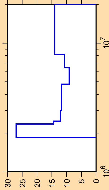
\Delta\sigma/\sigma vs. E for ^{175}\text{Tm}(n,ncont.)
