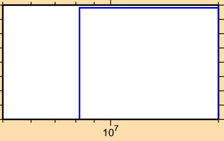
\sigma vs. E for ^{175}\text{Tm}(n,d)
