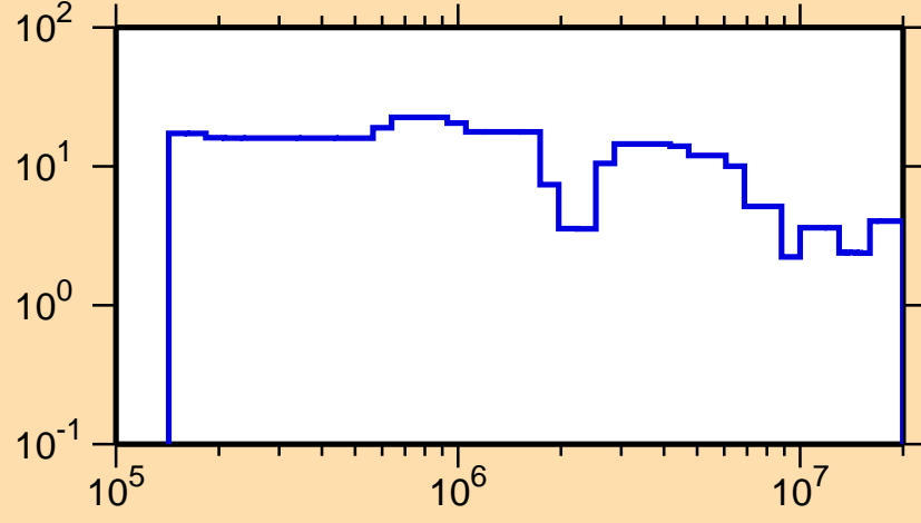
\Delta\sigma/\sigma vs. E for ^{176}\text{Tm}(n, tot.)
