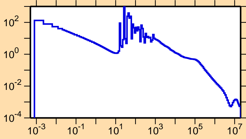
\sigma vs. E for ^{176}\text{Tm}(n,\gamma)
