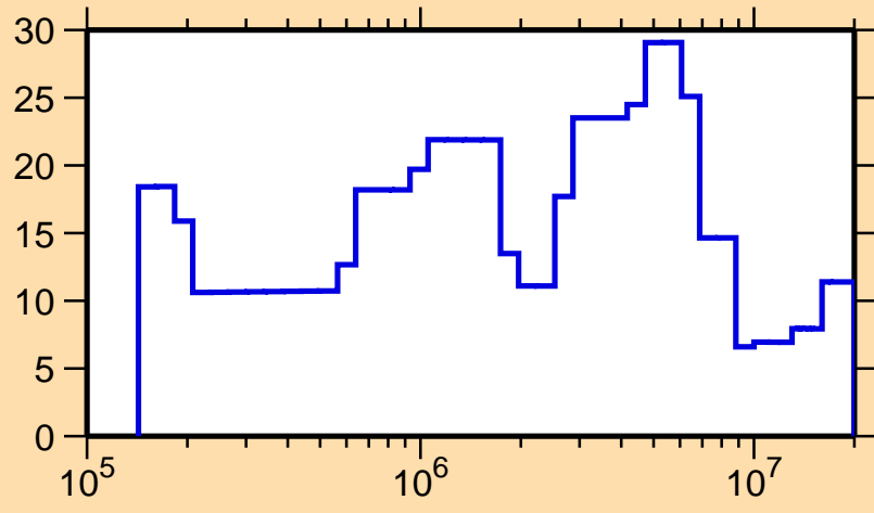
\Delta\sigma/\sigma vs. E for ^{176}\text{Tm}(n, el.)
