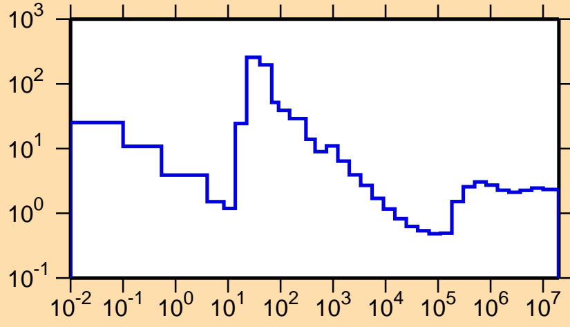
\sigma vs. E for ^{176}\text{Tm}(n,\text{nonel.})
