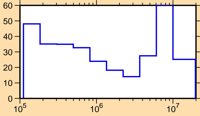
\Delta\sigma/\sigma vs. E for ^{176}\text{Tm}(n,n\text{cont.})
