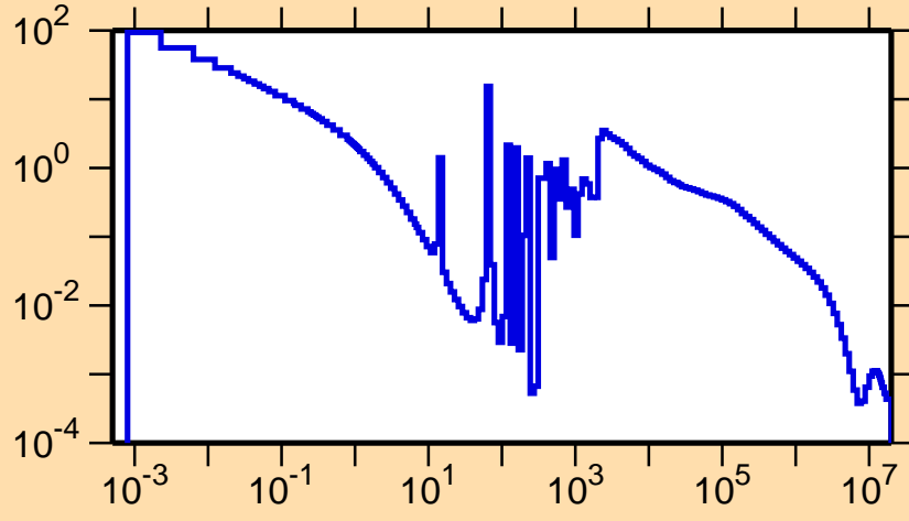
\sigma vs. E for ^{177}\text{Tm}(n,\gamma)
