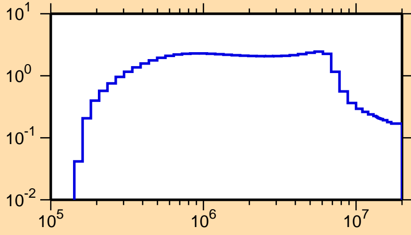
\sigma vs. E for ^{177}\text{Tm}(n,\text{inel.})
