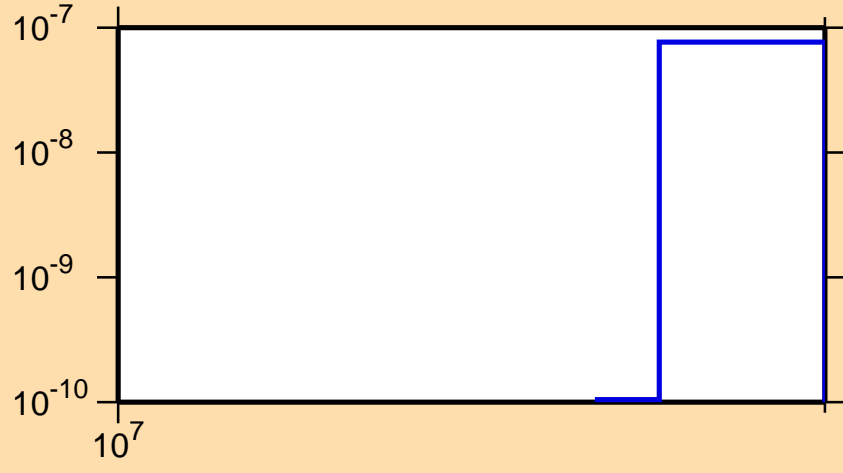
\sigma vs. E for ^{177}\text{Tm}(n,2np)
