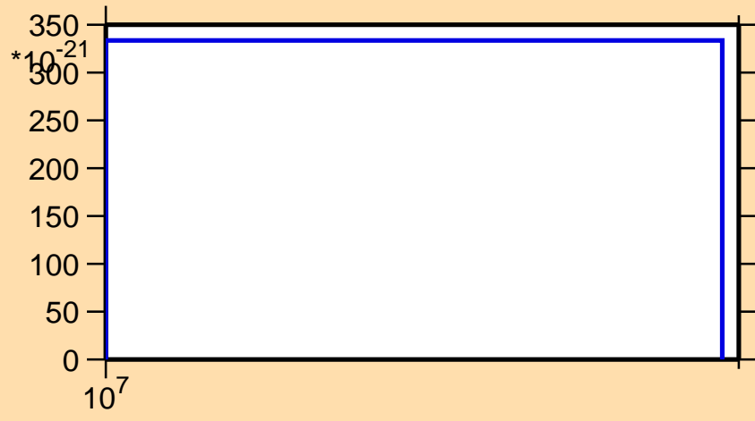
\sigma vs. E for ^{177}\text{Tm} (mt 42)
