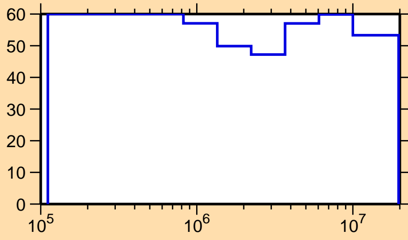
\Delta\sigma/\sigma vs. E for ^{177}\text{Tm}(n,n_1)
