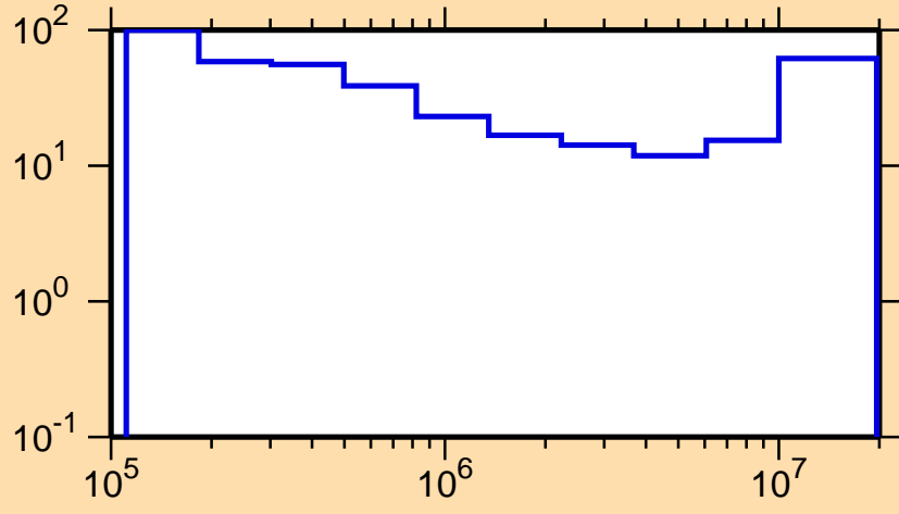
\Delta\sigma/\sigma vs. E for ^{177}\text{Tm}(n,n\text{cont.})
