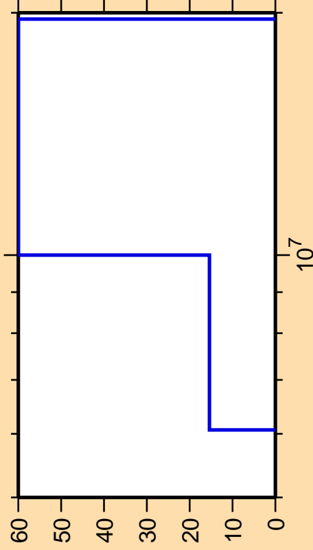
\Delta\sigma/\sigma vs. E for ^{177}\text{Tm}(n,n\text{cont.})
