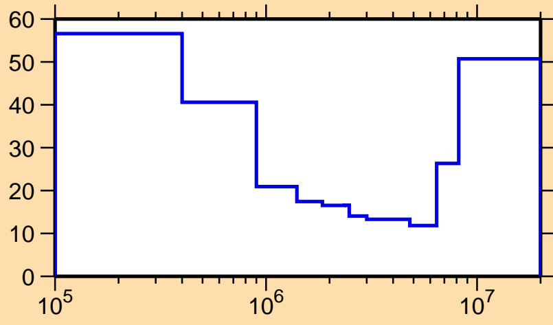
\Delta\sigma/\sigma vs. E for ^{177}\text{Tm}(n,n\text{cont.})
