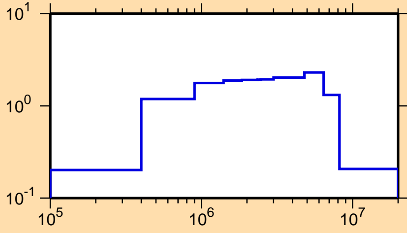
\sigma vs. E for ^{177}\text{Tm}(n,n\text{cont.})
