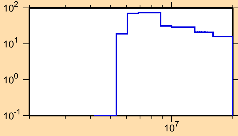
\Delta\sigma/\sigma vs. E for ^{178}\text{Tm}(n,p)
