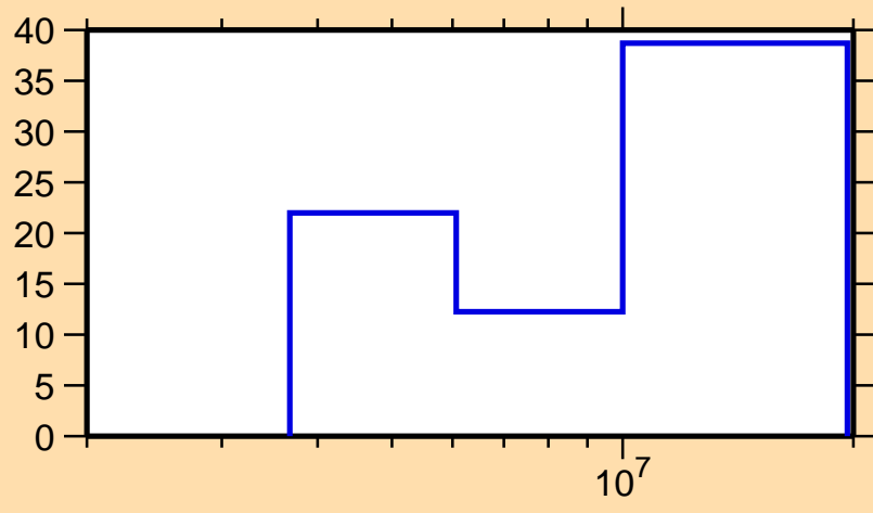
\Delta\sigma/\sigma vs. E for ^{178}\text{Tm}(n,2n)
