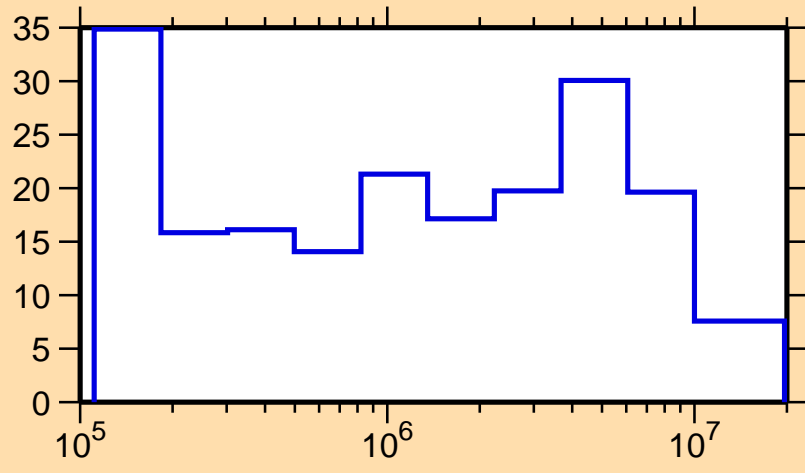
\Delta\sigma/\sigma vs. E for ^{178}\text{Tm}(n, el.)
