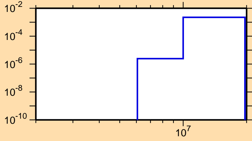
\sigma vs. E for ^{178}\text{Tm}(n,p)
