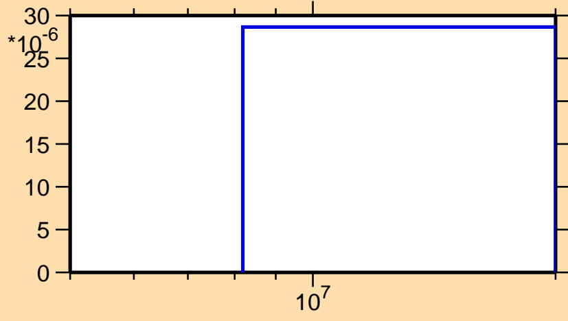
\sigma vs. E for ^{178}\text{Tm}(n,np)
