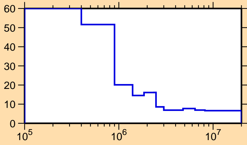
\Delta\sigma/\sigma vs. E for ^{178}\text{Tm}(n,\text{nonel.})
