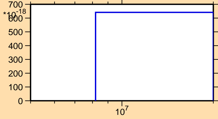
\sigma vs. E for ^{178}\text{Tm} (mt 11)
