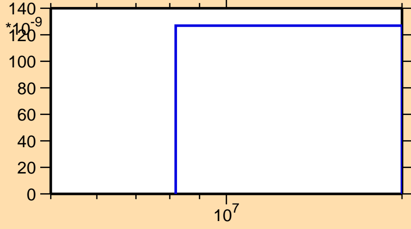
\sigma vs. E for ^{178}\text{Tm}(n,nt)
