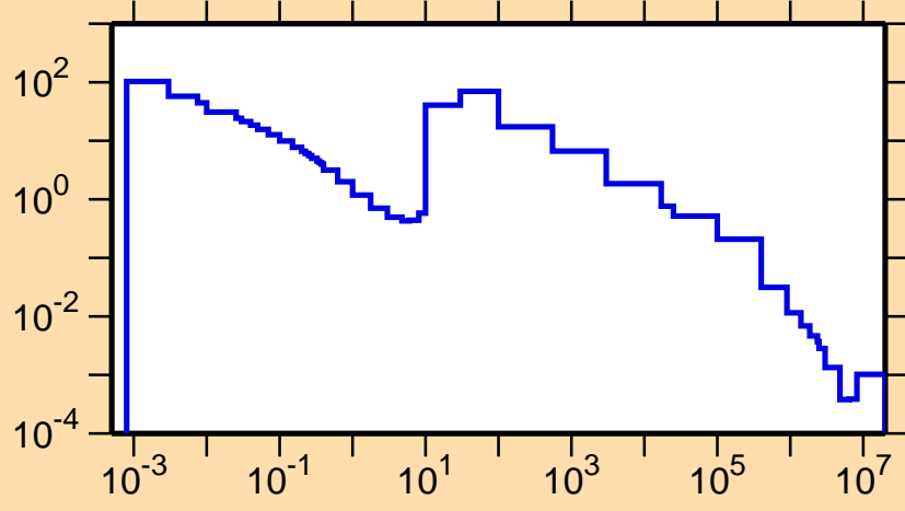
\sigma vs. E for ^{178}\text{Tm}(n,\gamma)
