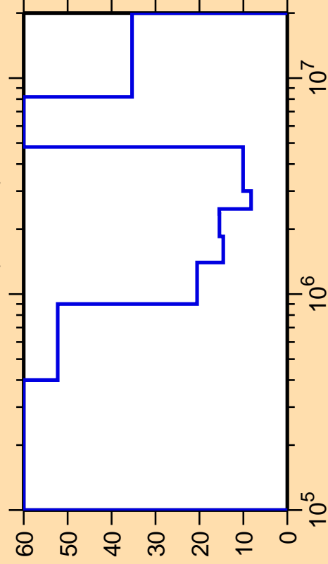
\Delta\sigma/\sigma vs. E for ^{178}\text{Tm}(n,\text{inel.})
