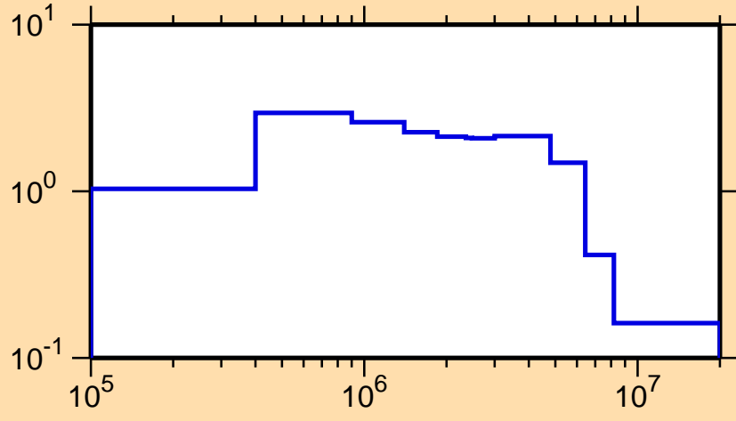
\sigma vs. E for ^{178}\text{Tm}(n,\text{inel.})
