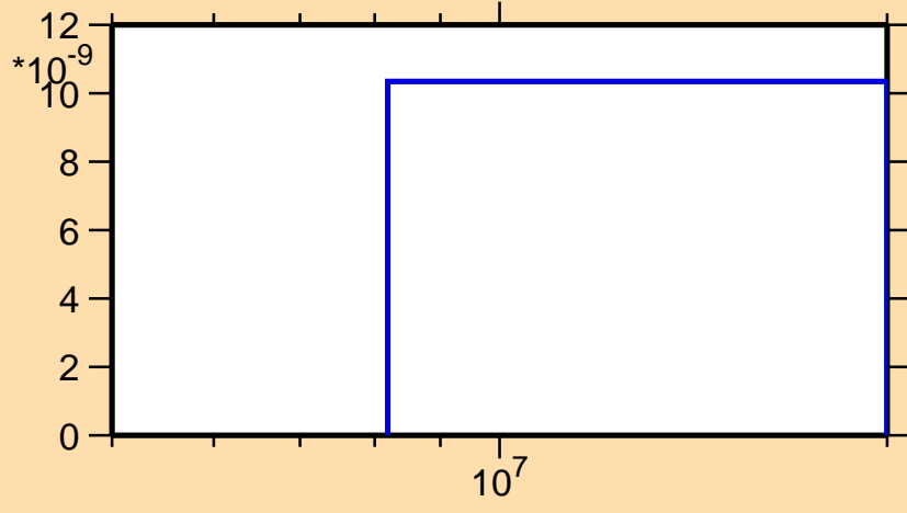
\sigma vs. E for ^{178}\text{Tm}(n,2np)
