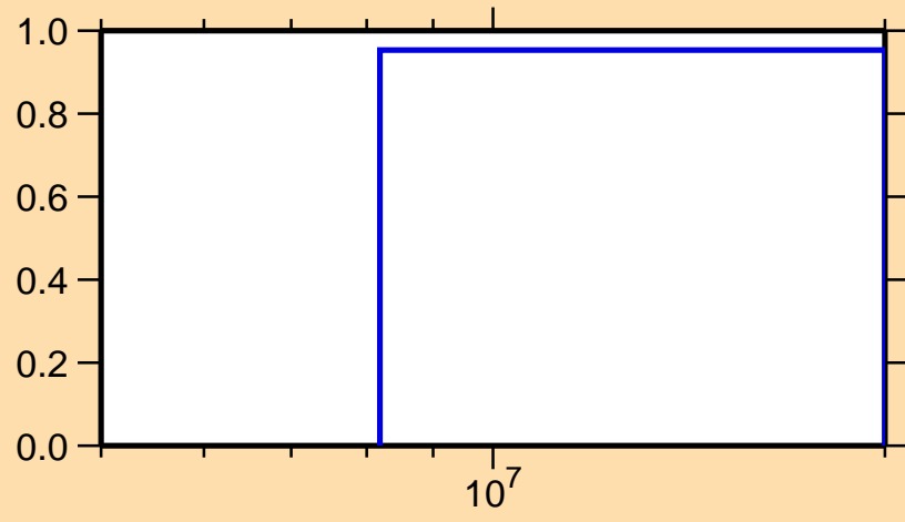
\sigma vs. E for ^{178}\text{Tm}(n,3n)
