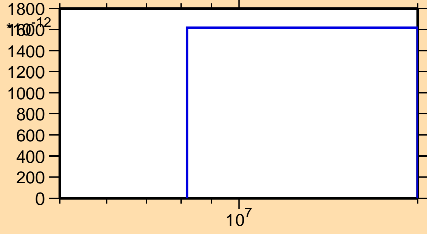
\sigma vs. E for ^{178}\text{Tm}(n,2n\alpha)
