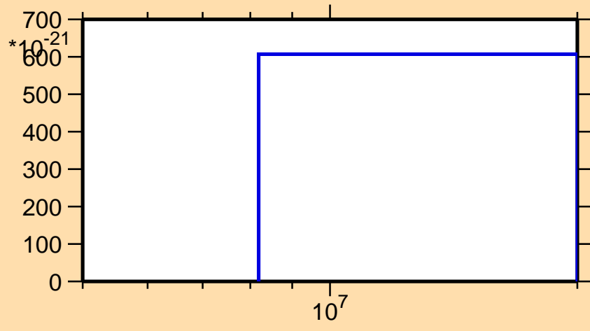
\sigma vs. E for ^{178}\text{Tm} (mt 42)
