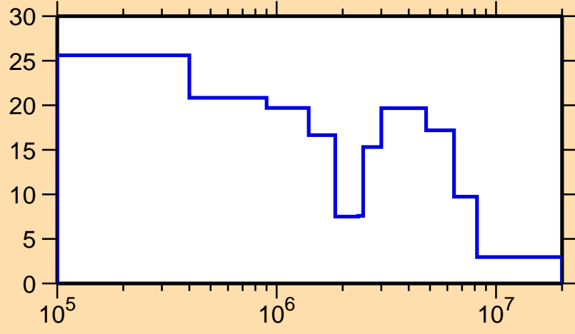
\Delta\sigma/\sigma vs. E for ^{178}\text{Tm}(n, \text{tot.})
