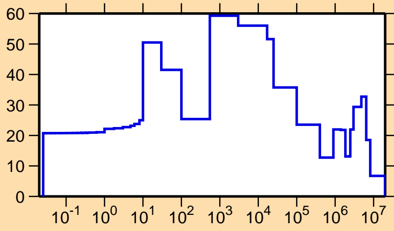
\Delta\sigma/\sigma vs. E for ^{178}\text{Tm}(n,\text{el.})
