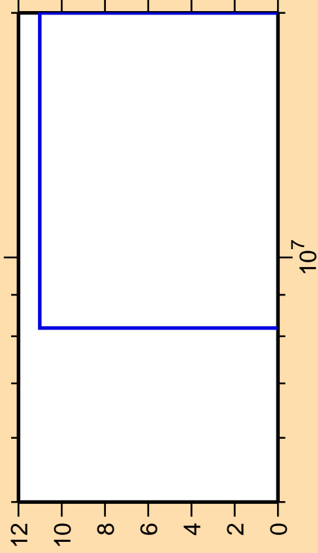
\Delta\sigma/\sigma vs. E for ^{178}\text{Tm}(n,3n)
