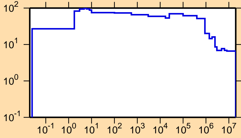
\Delta\sigma/\sigma vs. E for ^{178}\text{Tm}(n,\text{nonel.})
