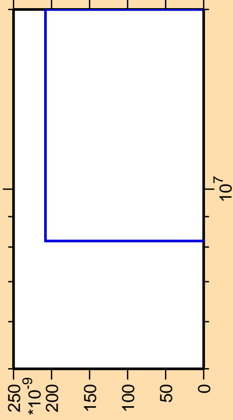
\Delta\sigma/\sigma vs. E for ^{178}\text{Tm} (mt 42)
