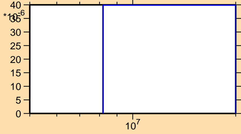
\sigma vs. E for ^{178}\text{Tm}(n,d)
