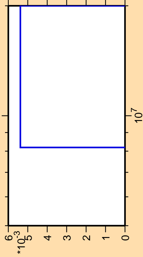
\Delta\sigma/\sigma vs. E for ^{178}\text{Tm} (mt 11)
