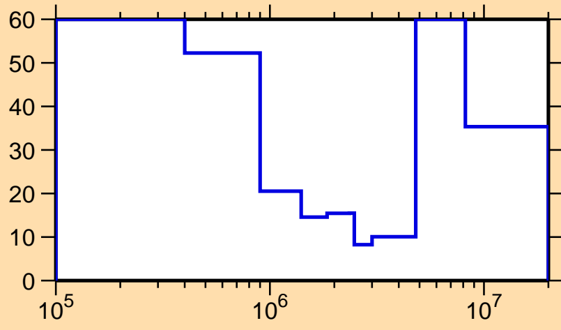
\Delta\sigma/\sigma vs. E for ^{178}\text{Tm}(n,\text{inel.})
