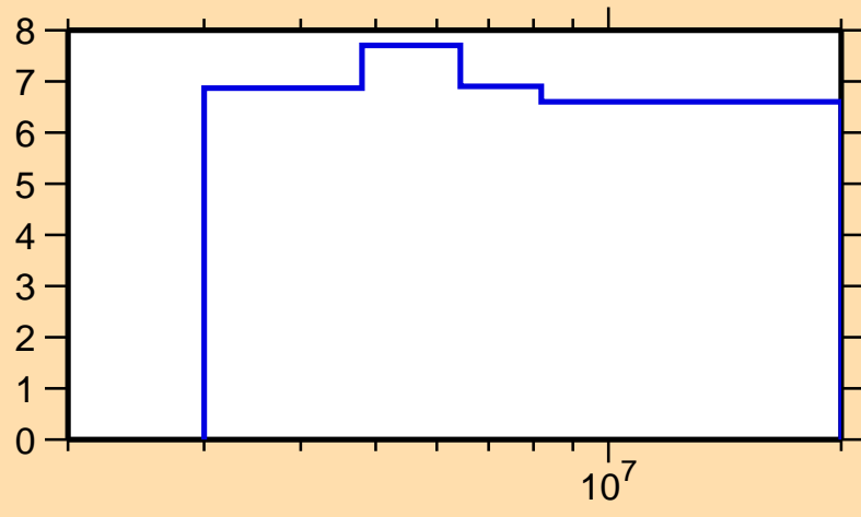
\Delta\sigma/\sigma vs. E for ^{178}\text{Tm}(n,\text{nonel.})
