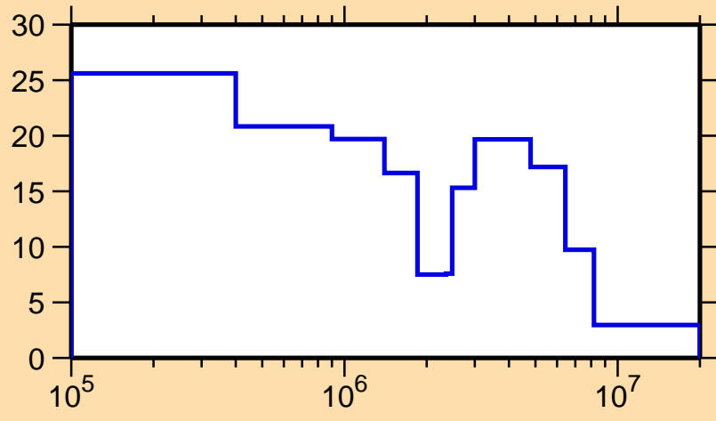
\Delta\sigma/\sigma vs. E for ^{178}\text{Tm}(n,\text{tot.})
