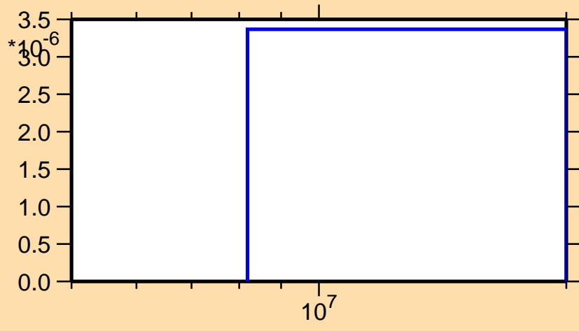
\sigma vs. E for ^{178}\text{Tm}(n,n\alpha)
