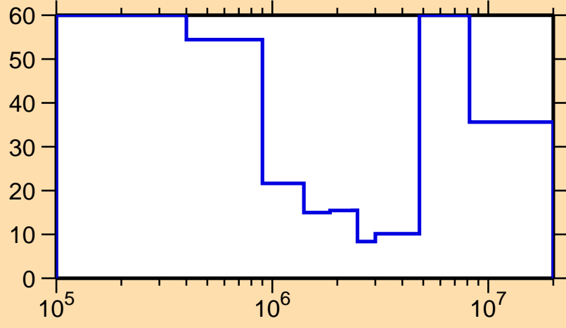
\Delta\sigma/\sigma vs. E for ^{178}\text{Tm}(n,n\text{cont.})
