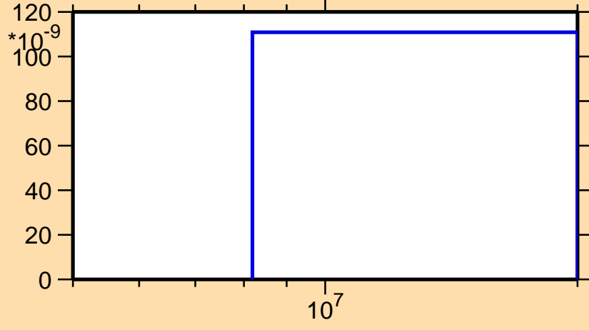
\sigma vs. E for ^{178}\text{Tm}(n,\text{nd})
