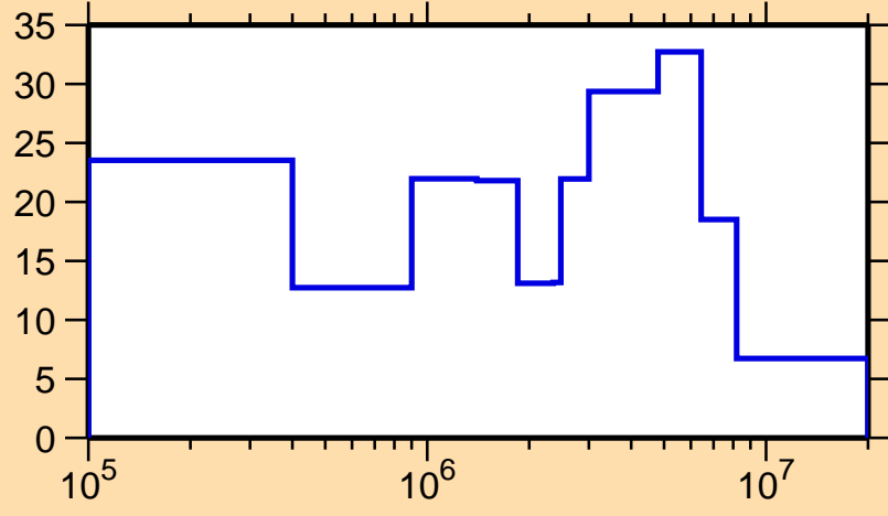
\Delta\sigma/\sigma vs. E for ^{178}\text{Tm}(n, el.)
