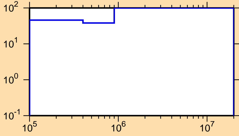
\Delta\sigma/\sigma vs. E for ^{178}\text{Tm}(n,n_1)
