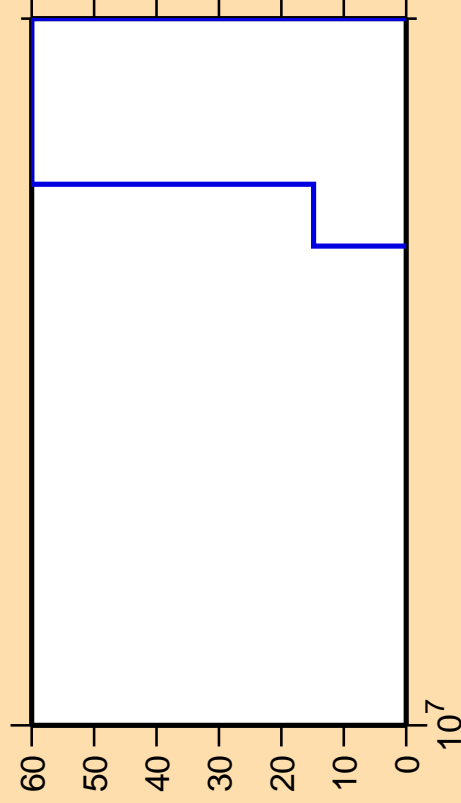
\Delta\sigma/\sigma vs. E for ^{227}\text{U} (mt117)
