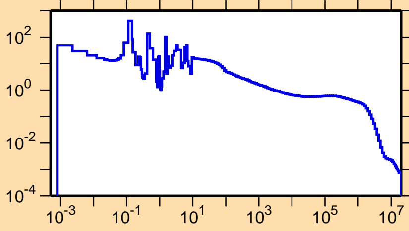
\sigma vs. E for ^{227}\text{U}(n,\gamma)
