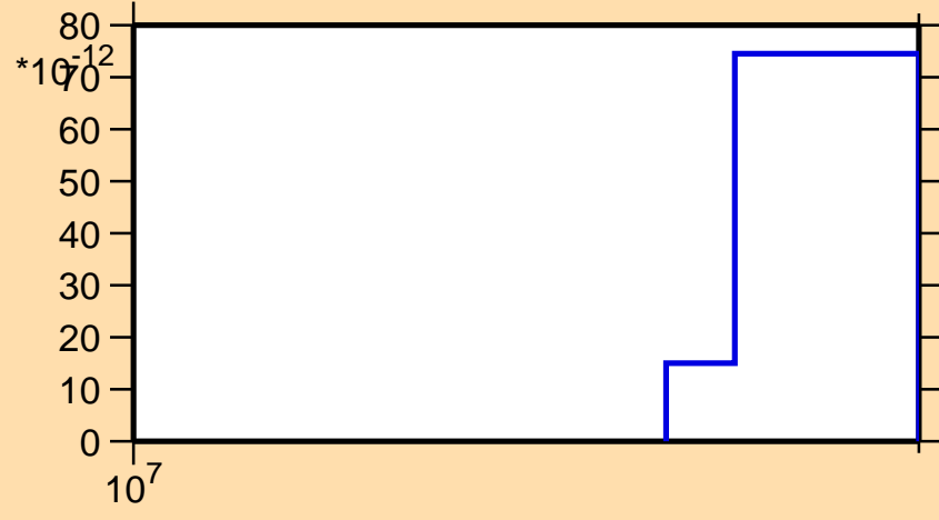
\sigma vs. E for ^{227}\text{U} (mt117)
