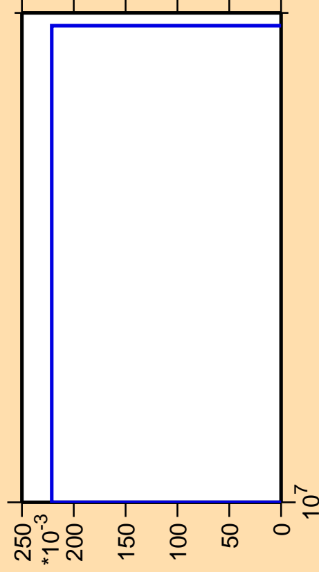
\Delta\sigma/\sigma vs. E for ^{227}\text{U} (mt 34)
