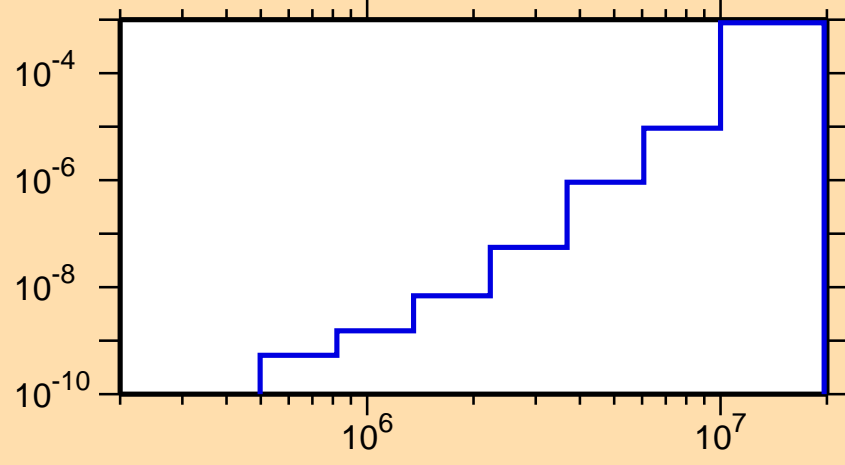
\sigma vs. E for ^{227}\text{U}(n,n\alpha)
