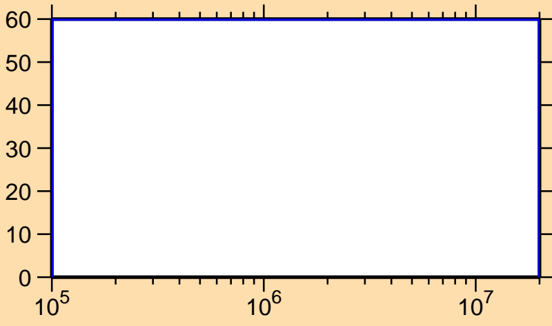
\Delta\sigma/\sigma vs. E for ^{227}\text{U}(n,inel.)
