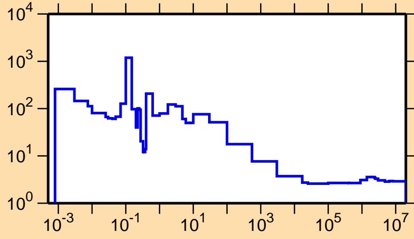
\sigma vs. E for ^{227}\text{U}(n,\text{nonel.})
