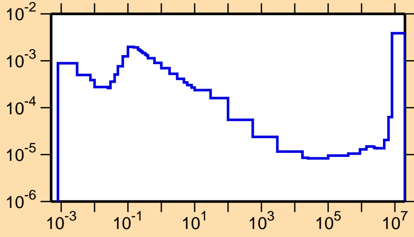
\sigma vs. E for ^{227}\text{U}(n,\alpha)
