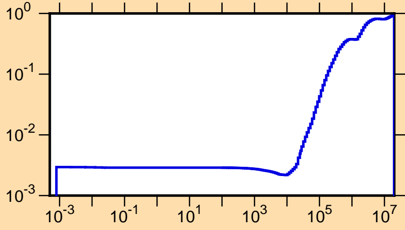
\mu vs. E for ^{228}\text{U}(\text{mt251})
