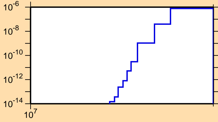
\sigma vs. E for ^{231}\text{U}(n,2np)
