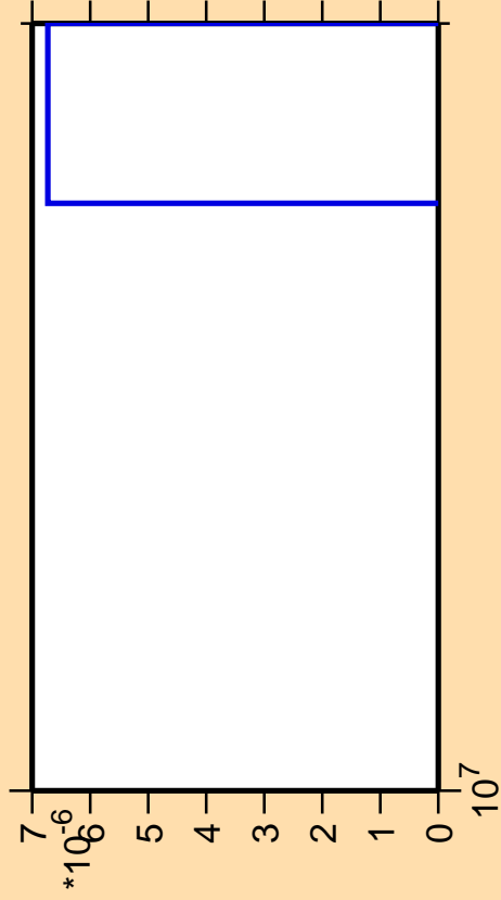
\Delta\sigma/\sigma vs. E for ^{231}\text{U} (mt 42)
