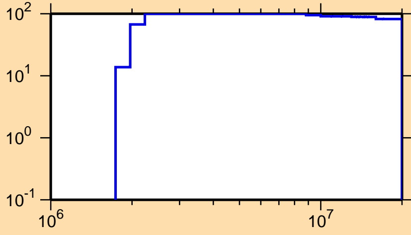
\Delta\sigma/\sigma vs. E for ^{231}\text{U}(n,p)
