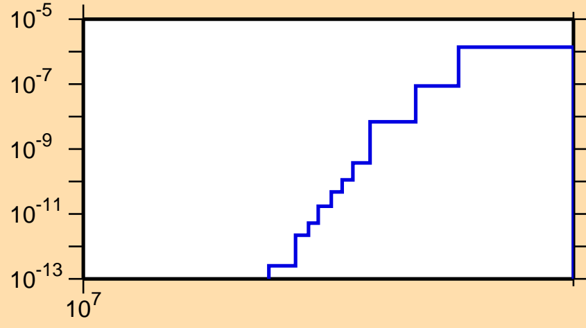
\sigma vs. E for ^{231}\text{U}(n,nd)
