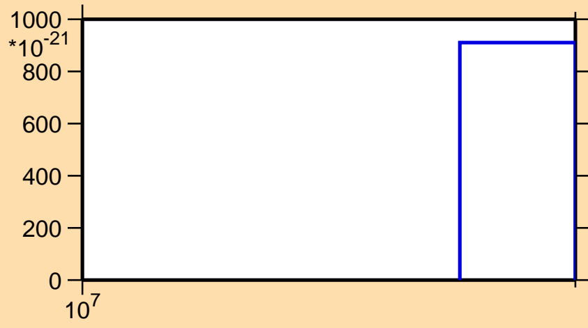
\sigma vs. E for ^{231}\text{U} (mt 42)
