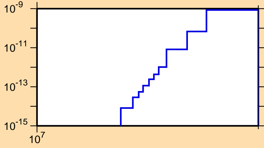
\sigma vs. E for ^{231}\text{U}(n,\text{He3})
