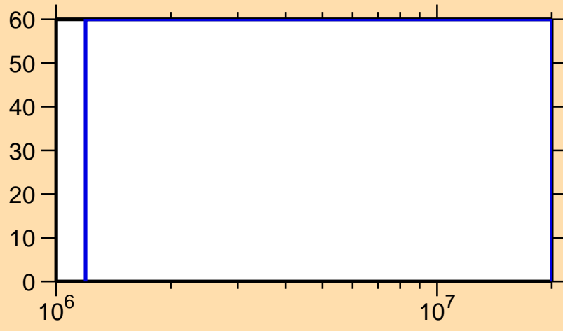
\Delta\sigma/\sigma vs. E for ^{231}\text{U}(n,n\text{cont.})
