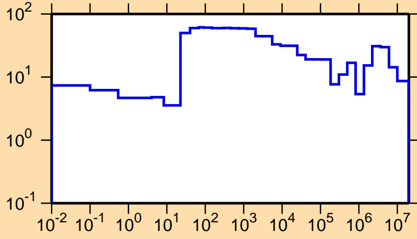
\Delta\sigma/\sigma vs. E for ^{231}\text{U}(n,tot.)
