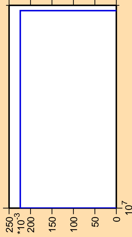
\Delta\sigma/\sigma vs. E for ^{231}\text{U}(n,3n\alpha)
