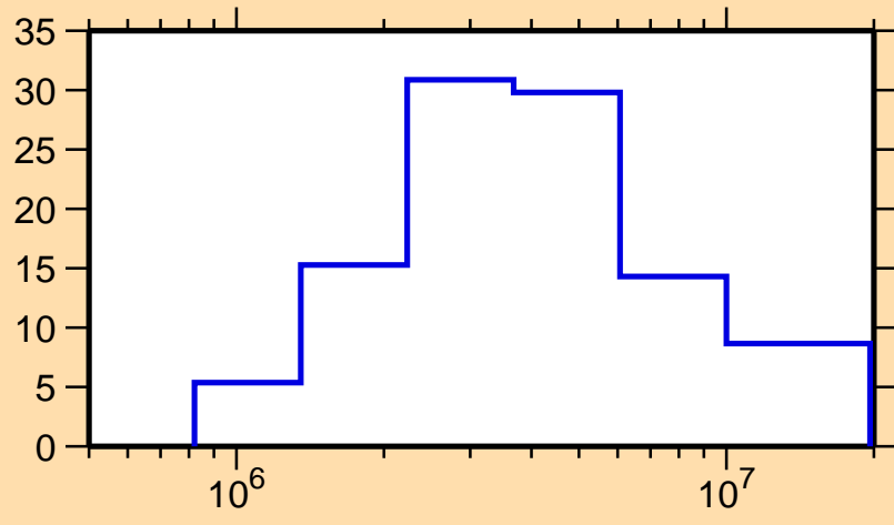
\Delta\sigma/\sigma vs. E for ^{231}\text{U}(n, tot.)
